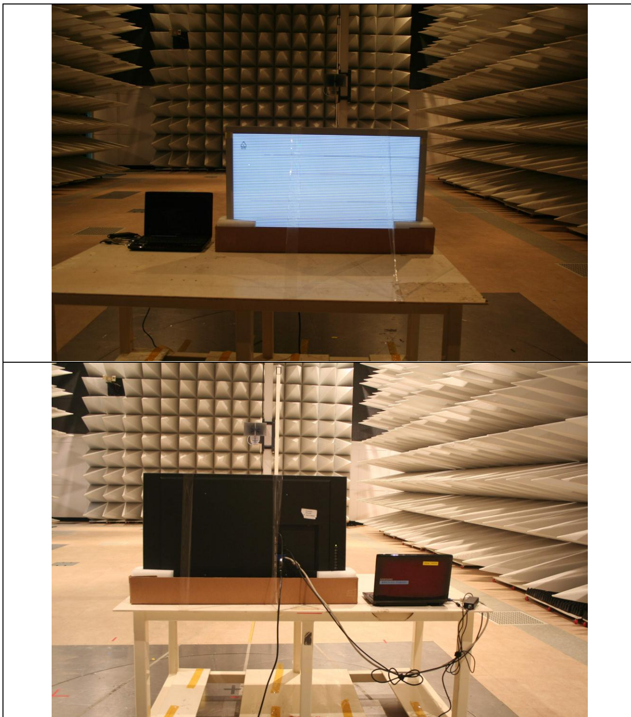
Figure 3. Photo of Radiated emission test setup for VGA Mode, 1.0 GHz to 2.0 GHz:
