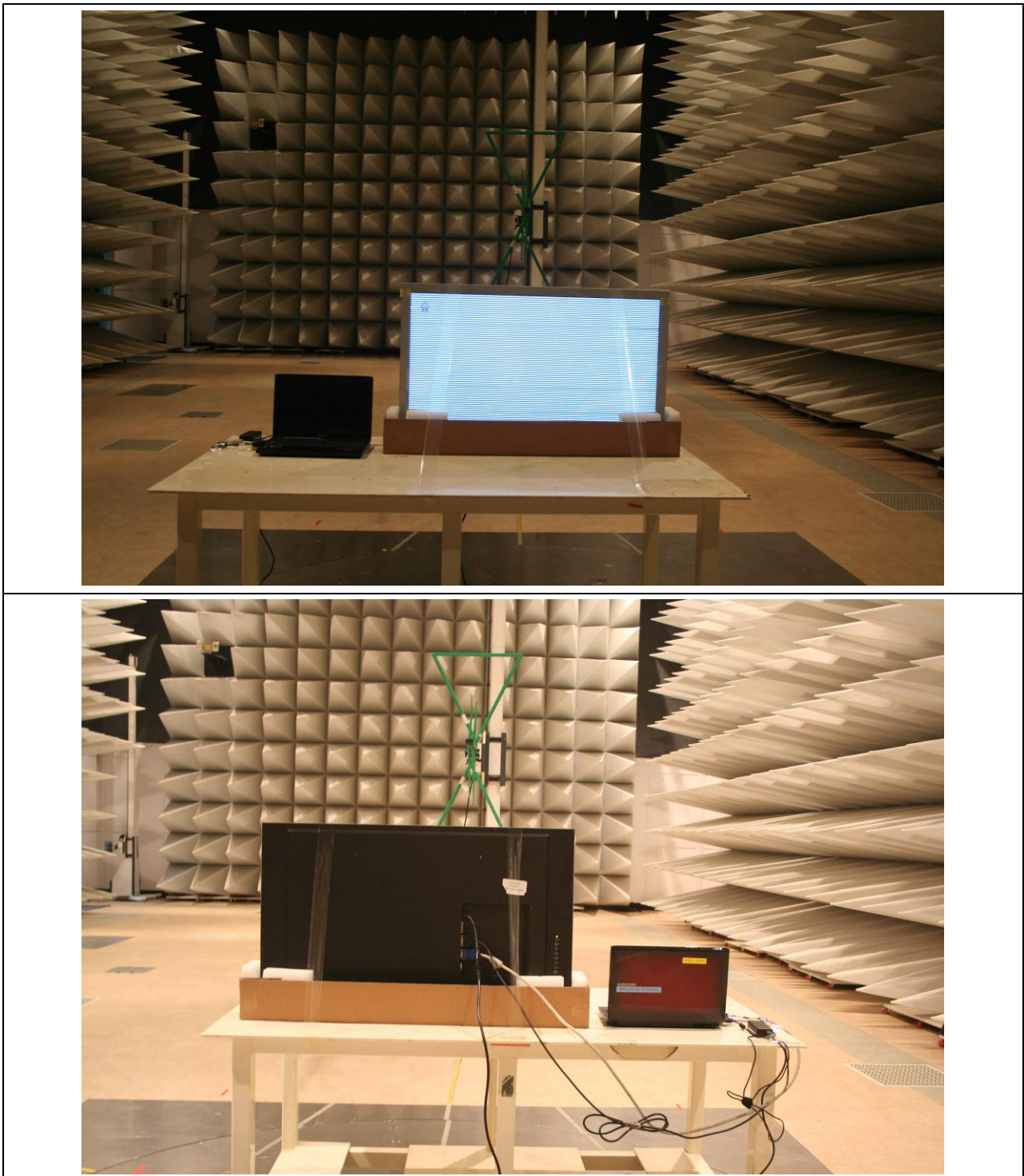
Figure 2. Photo of Radiated emission test setup for VGA Mode, 30 to 1000MHz:
