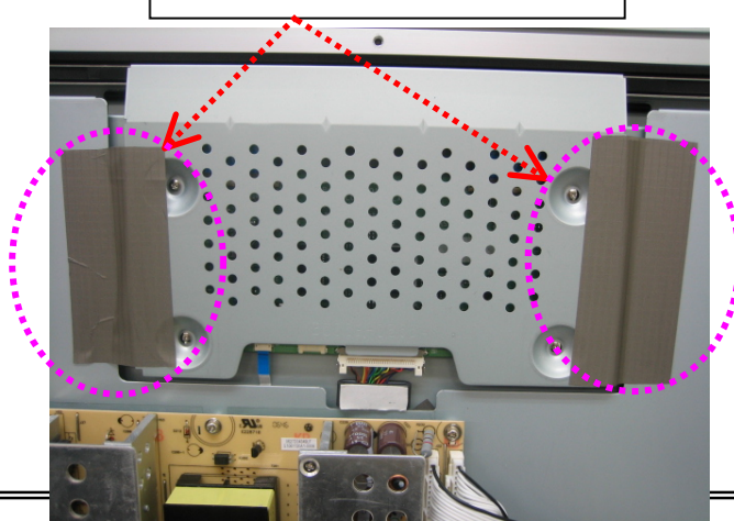
Attach the EMI tape
