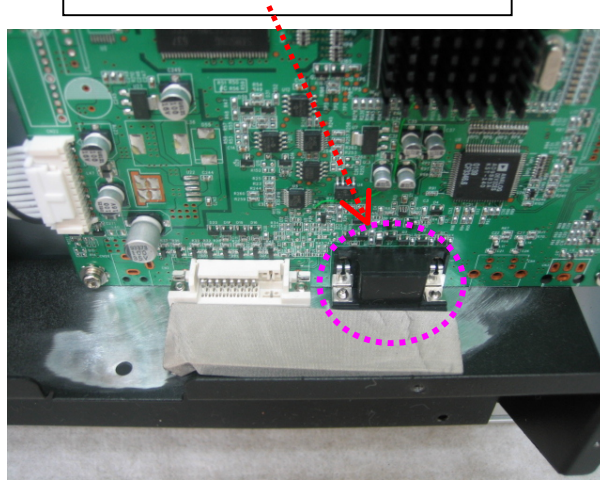
Attach the back gasket
