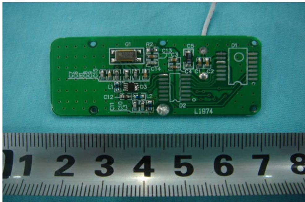
PCB-Front View
