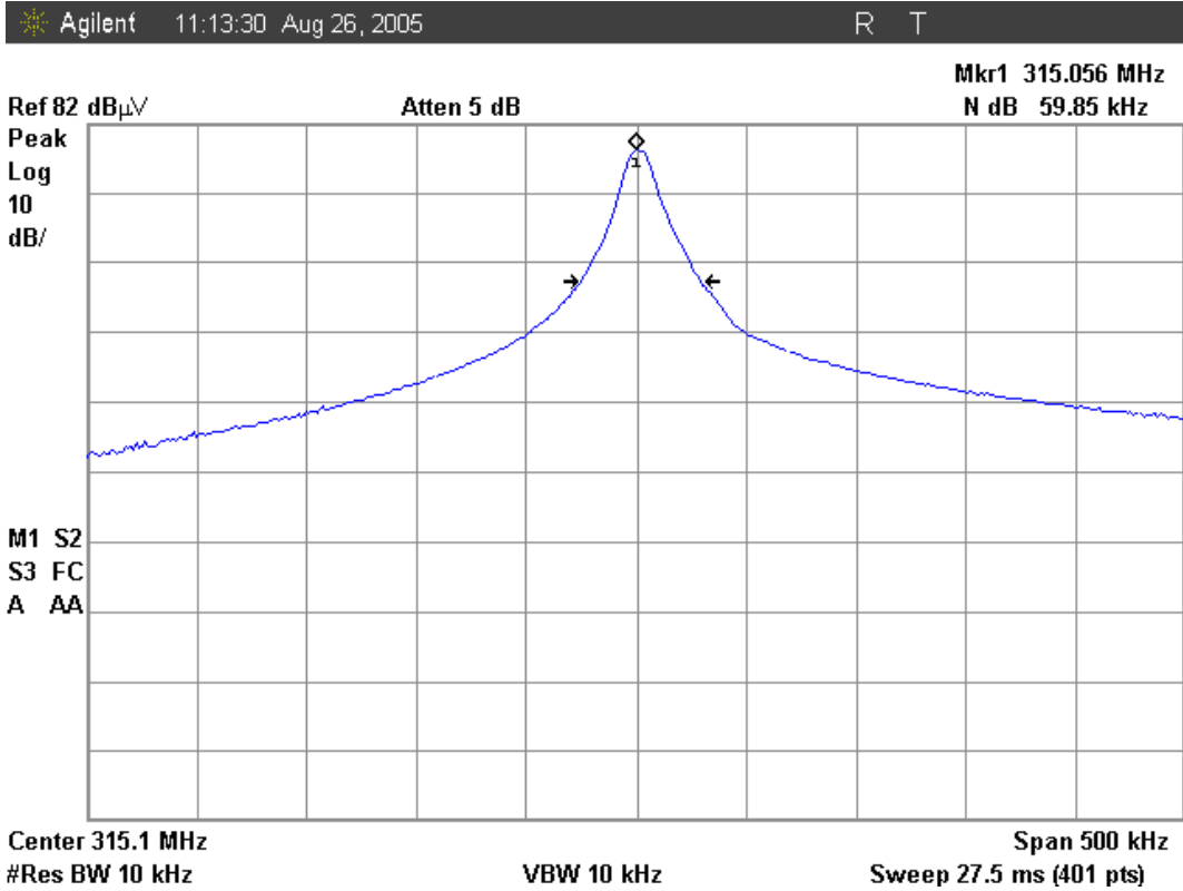
Figure 2: Measured value of the Occupied bandwidth
