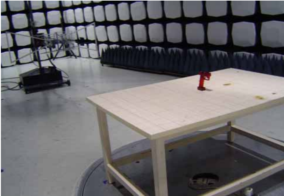
Radiation Emission Test setup
