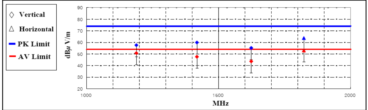
< Fig 6. Radiated emission result (1 000 MHz ~ 2 000 MHz)>
