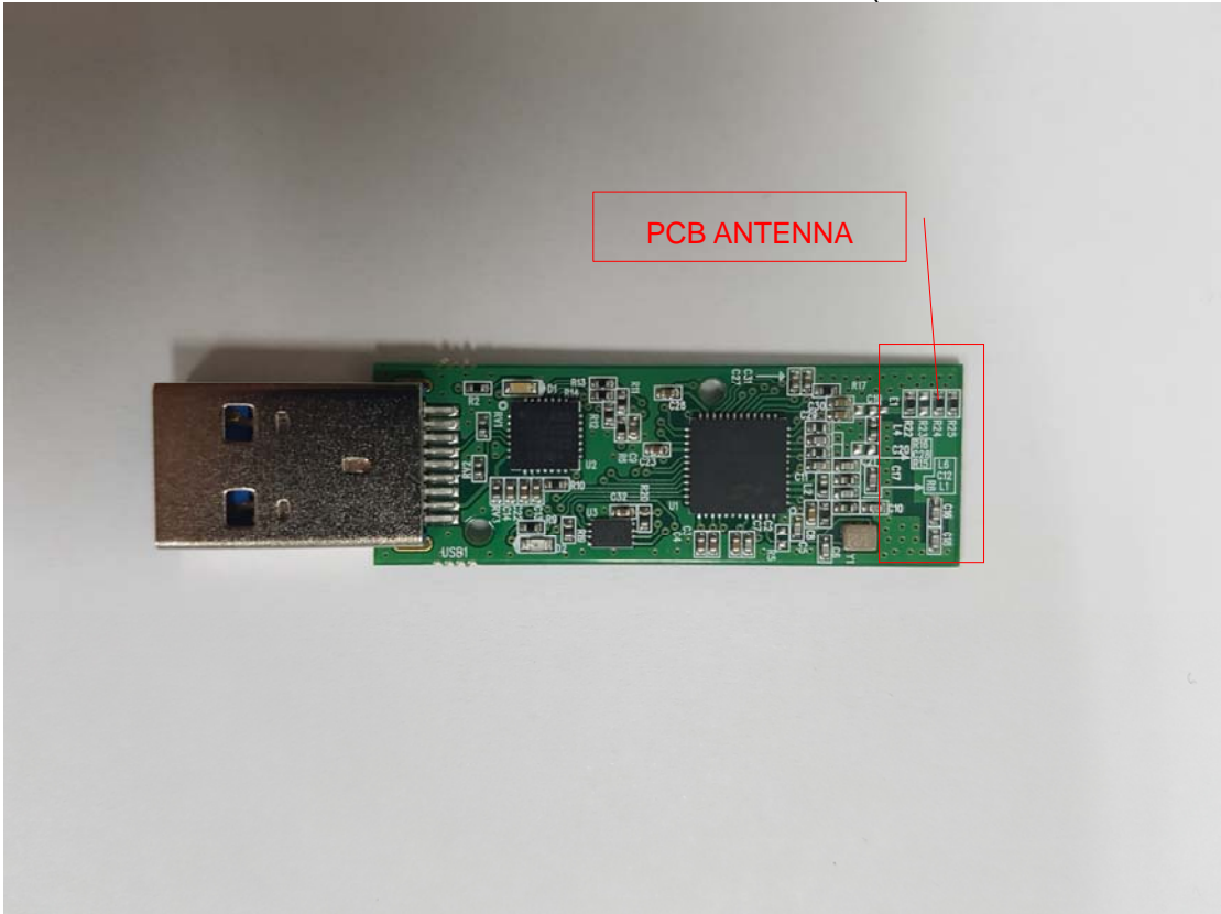
Figure 4 Internal View (I/O Board, Front View)
