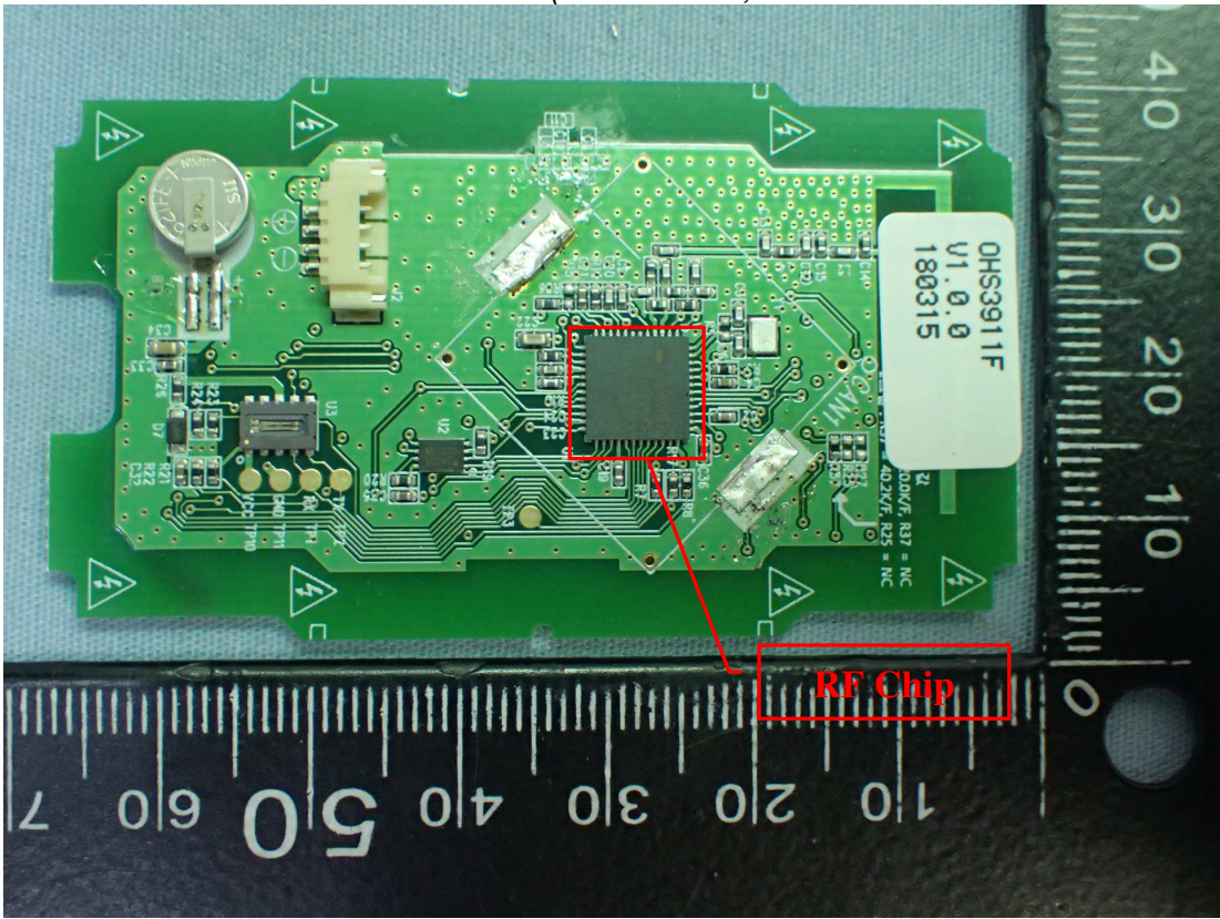
Figure 11 Internal View (Main Board, Front View/Removed Shielded Case)
