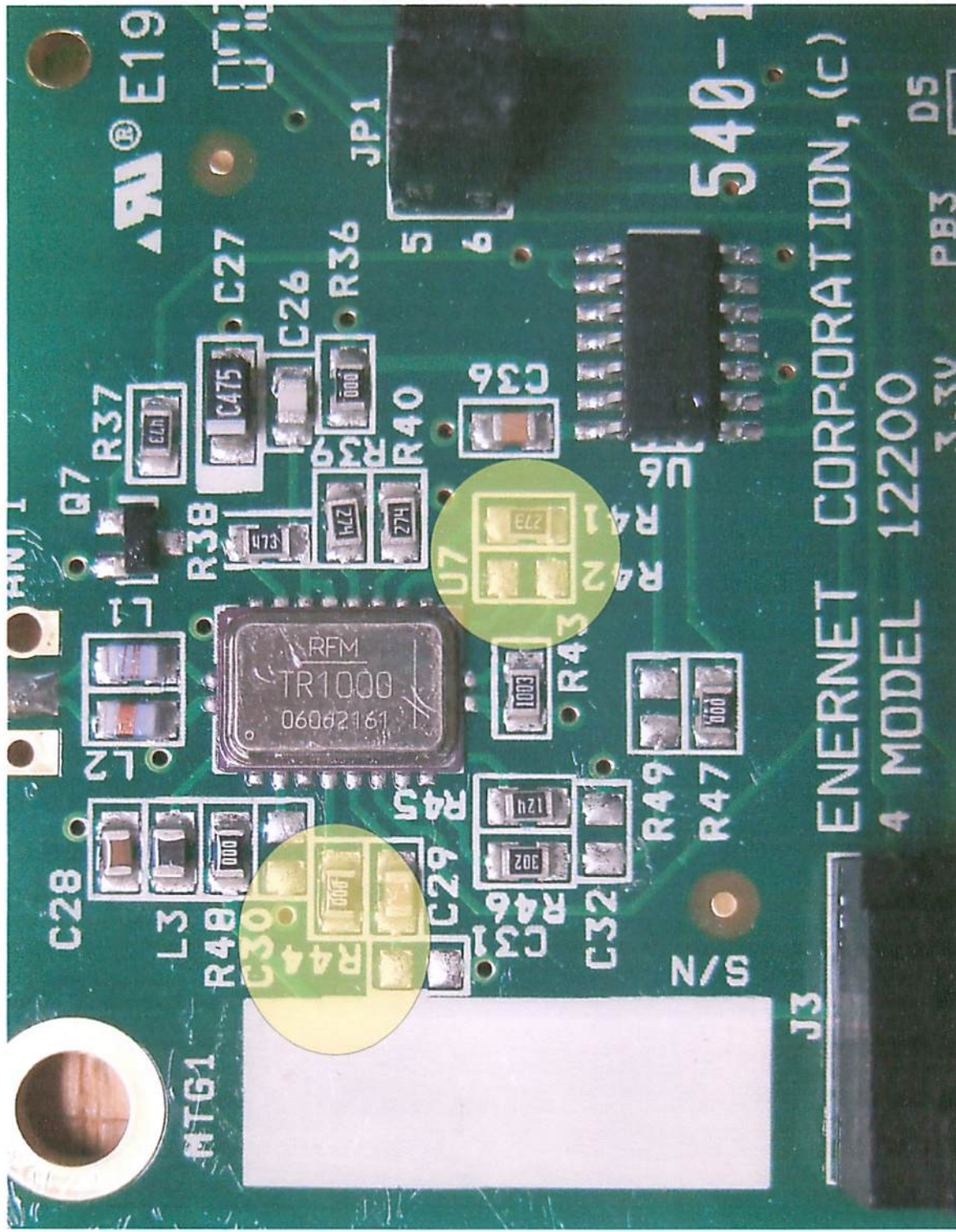
Fig. 2, Original Receiver Components
