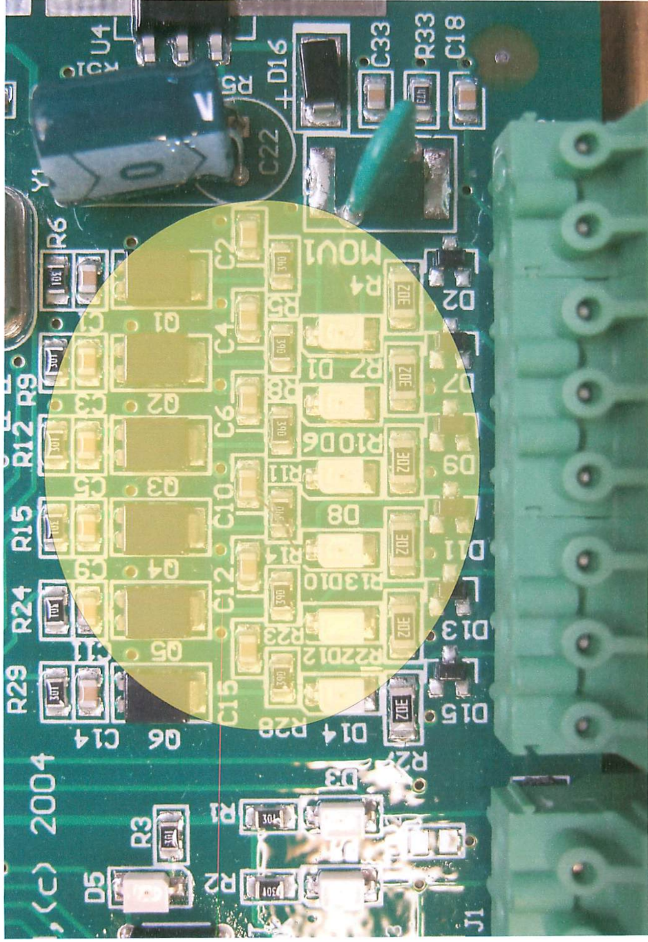
Fig. 5, Original Drive Circuit
