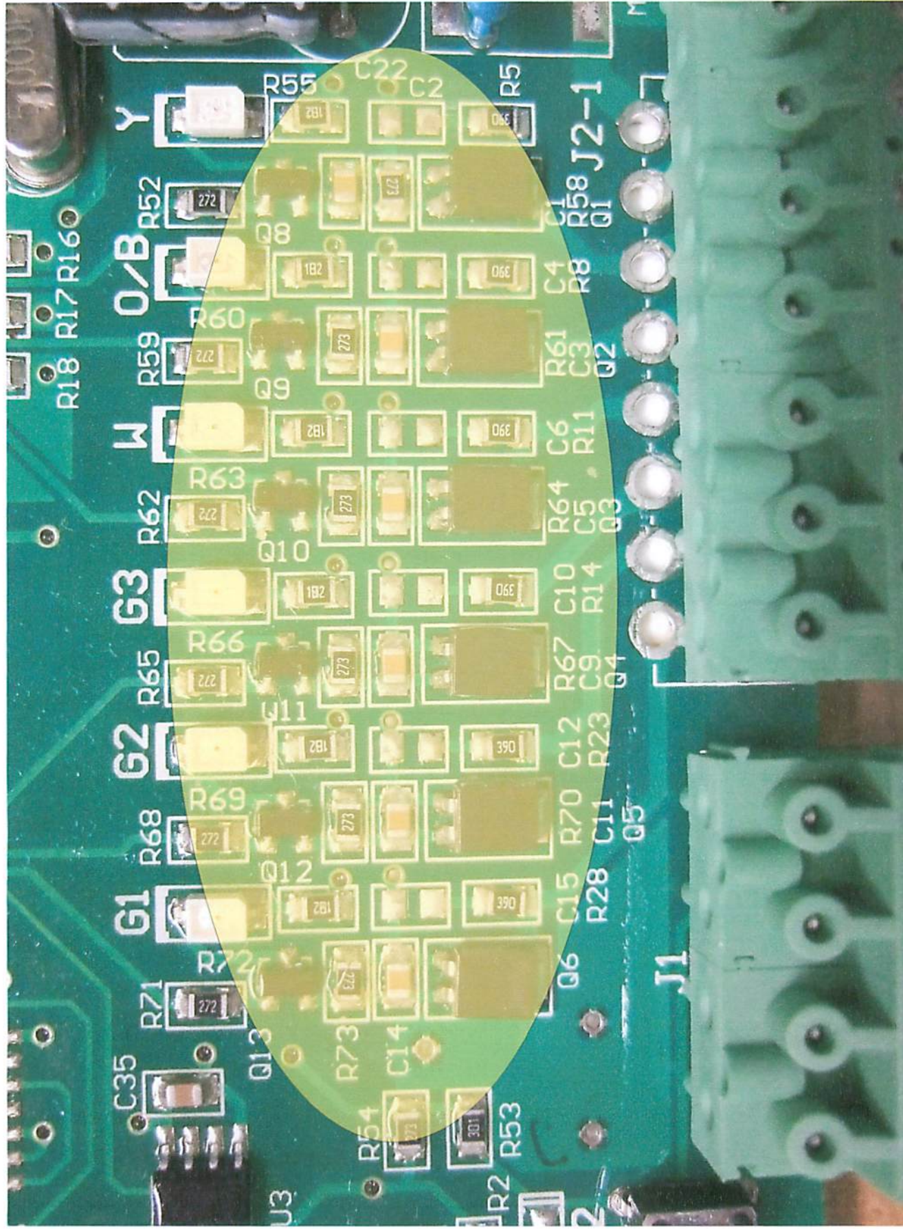
Fig. 6, Modified Drive Circuit
