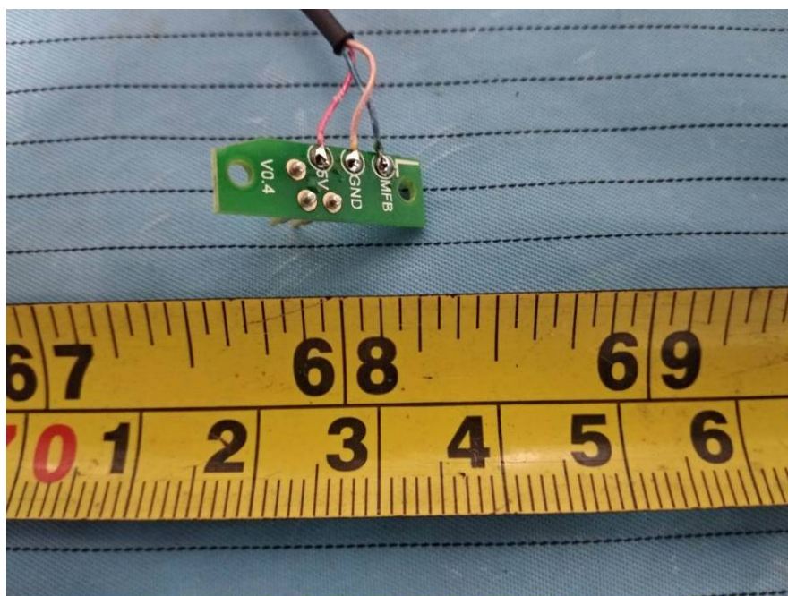
Left Charging Board Top View
