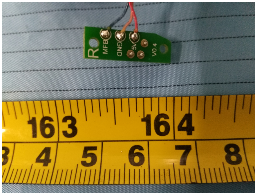
Right Charging Board Top View
