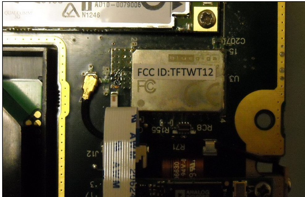
Figure 1: PCB - Front
