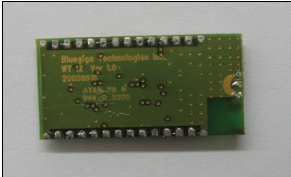
Figure 3: PCB – Back
