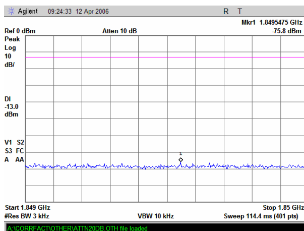
Plot 8.3.16 Spurious emission measurements in 1849 - 1850 MHz range at high carrier frequency
