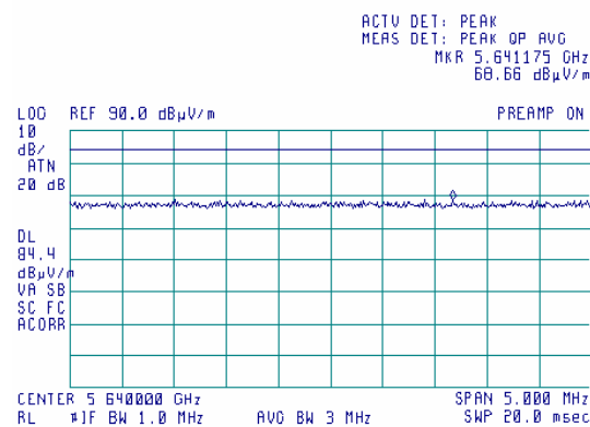
Plot 8.4.27 Radiated emission measurements at the third harmonic of high carrier frequency
