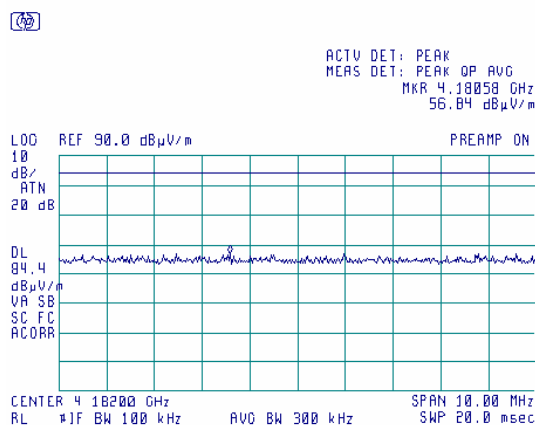
Plot 7.4.30 Radiated emission measurements at the fifth harmonic of high carrier frequency
