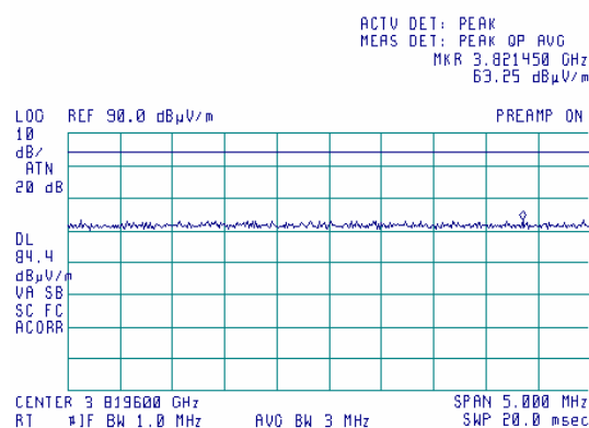
Plot 8.4.25 Radiated emission measurements at the third harmonic of low carrier frequency
