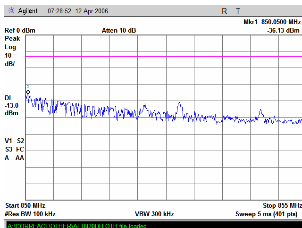
Plot 7.3.19 Spurious emission measurements in 850 - 855 MHz range at high carrier frequency
