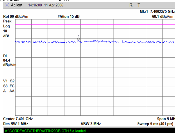
Plot 8.4.29 Radiated emission measurements at the forth harmonic of mid carrier frequency
