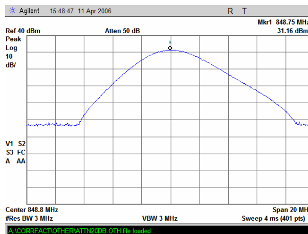
Plot 7.2.7 Occupied bandwidth test result at high frequency, reference level
