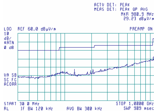
Plot 8.4.8 Radiated emission measurements from 30 to 1000 MHz at the mid carrier frequency
