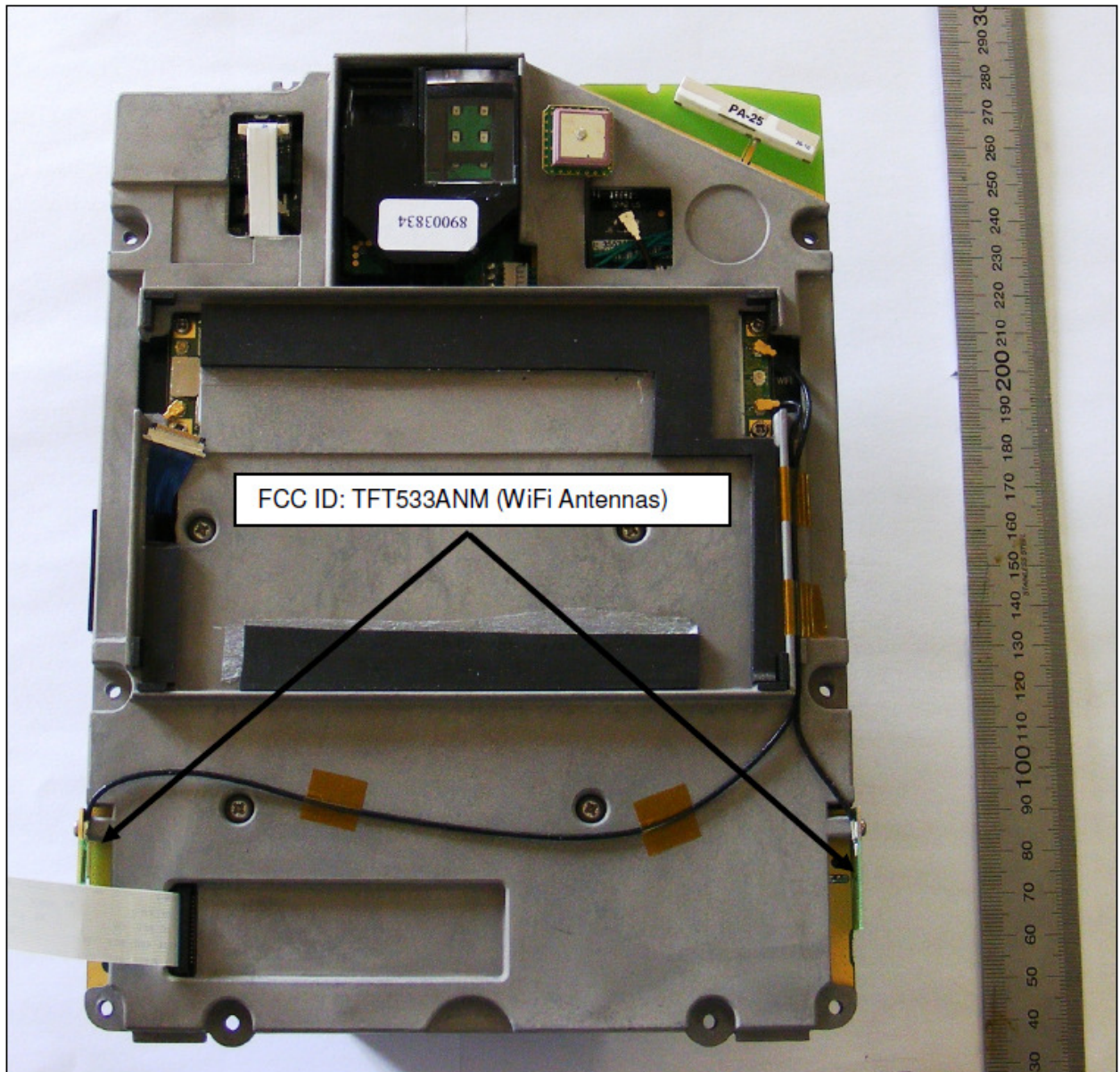
Figure 3: WiFi Antenna Locations
