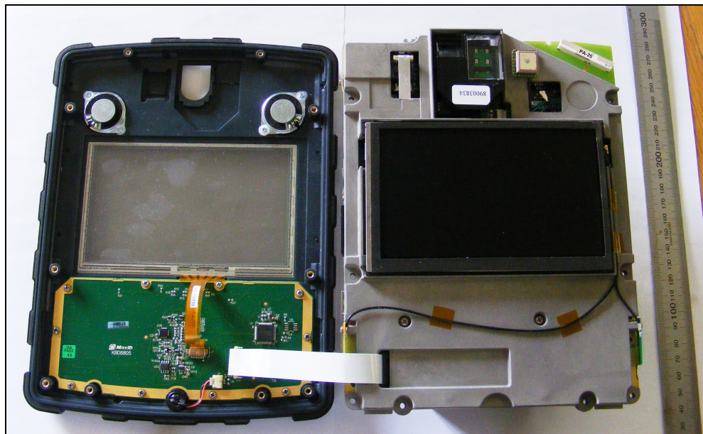
Figure 1: PCBs – Installed, Front
