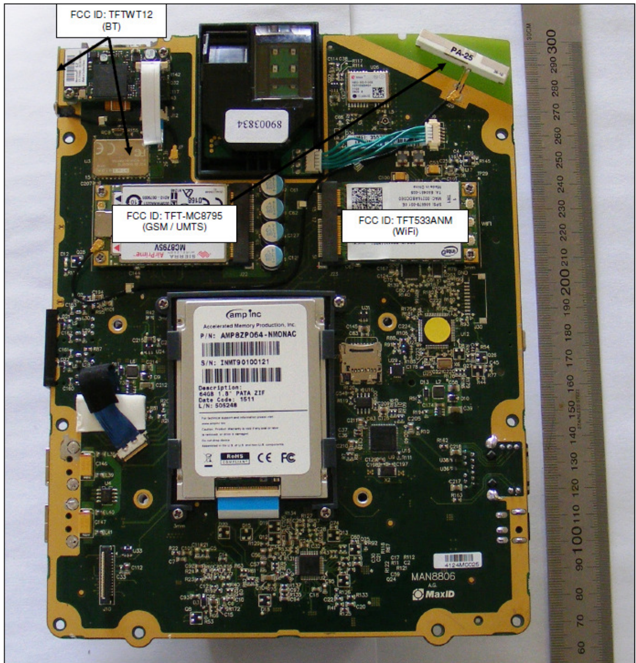
Figure 2: Main PCB – Front
