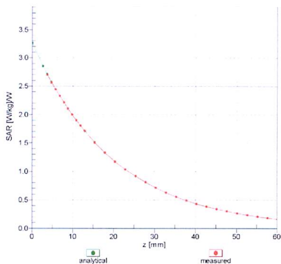
f = 835 MHz, WGLS R9 (M_convF)
