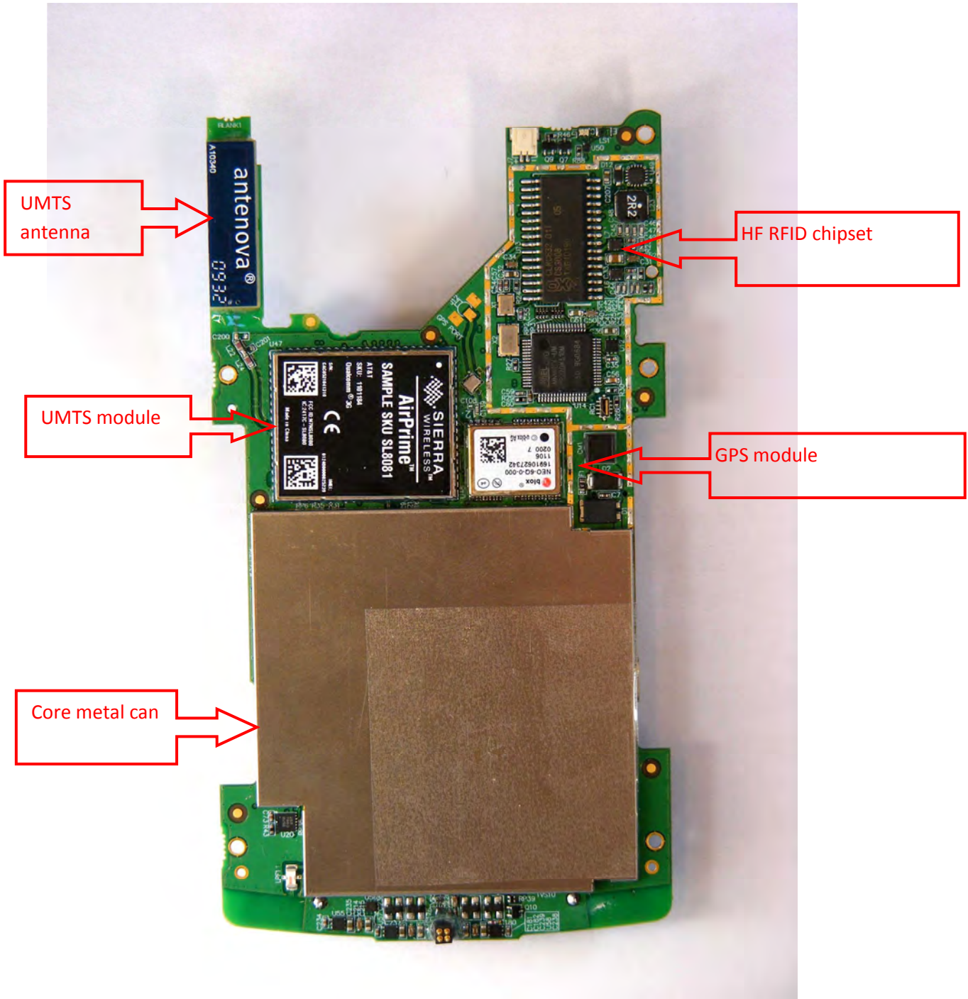
Figure 1: main board top view.
