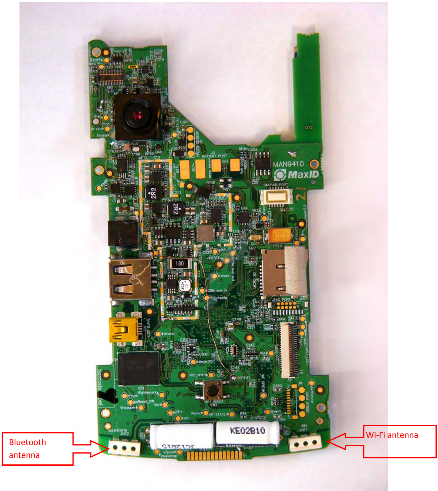
Figure 3: main board bottom view
