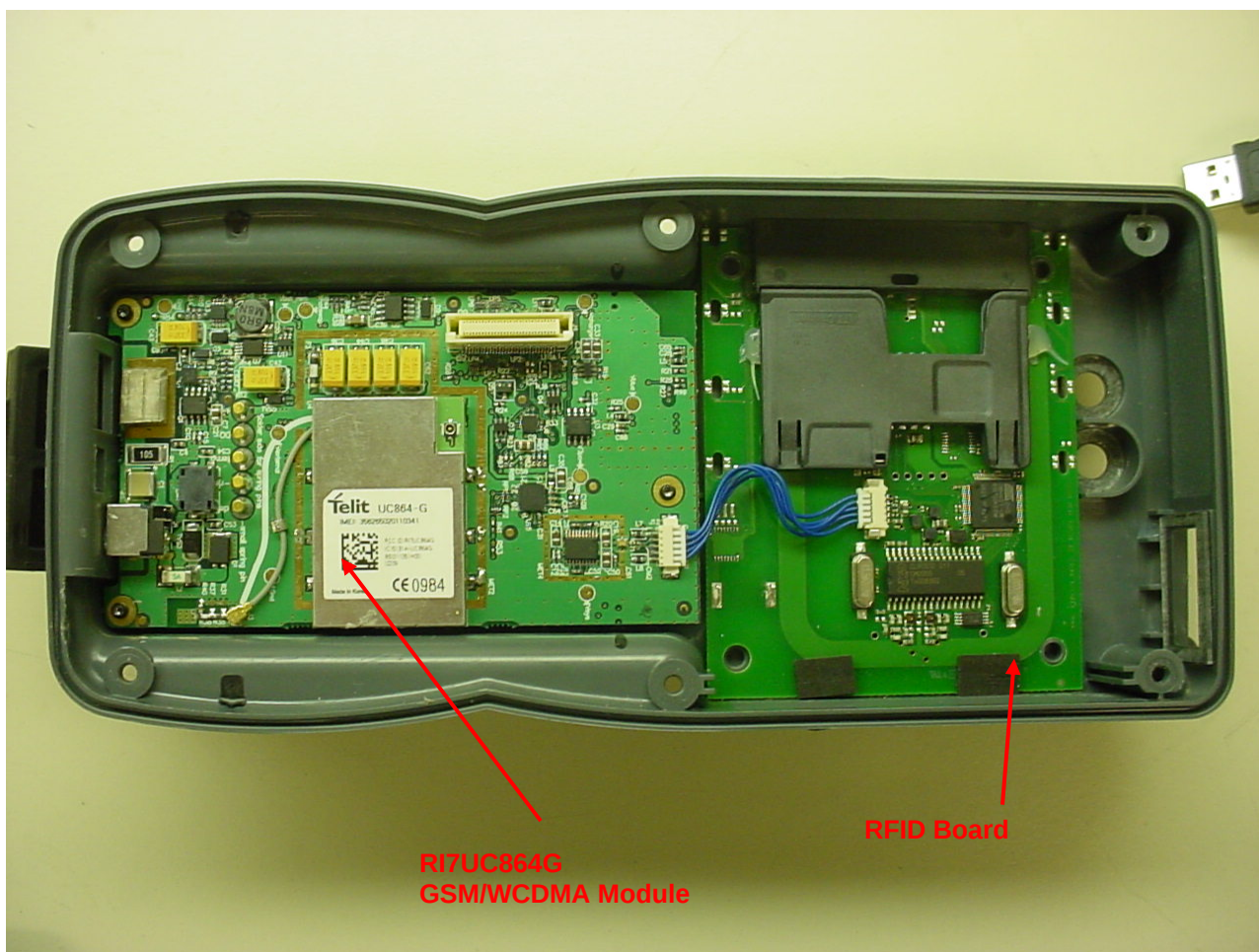
Figure 3: RFID Board and GSM/WCDMA Module Placement
