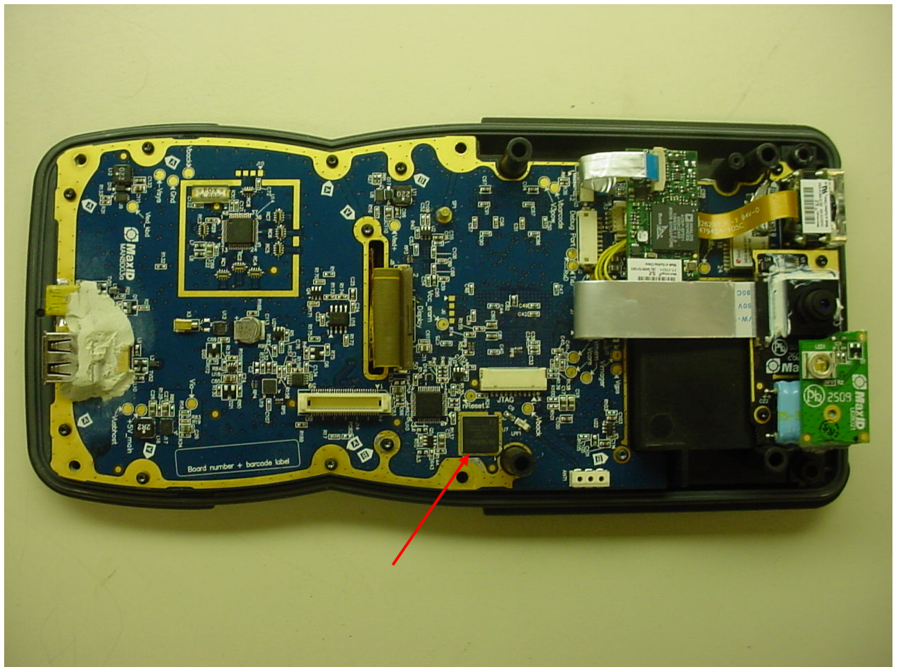
Figure 2: 802.11 Module Placement
