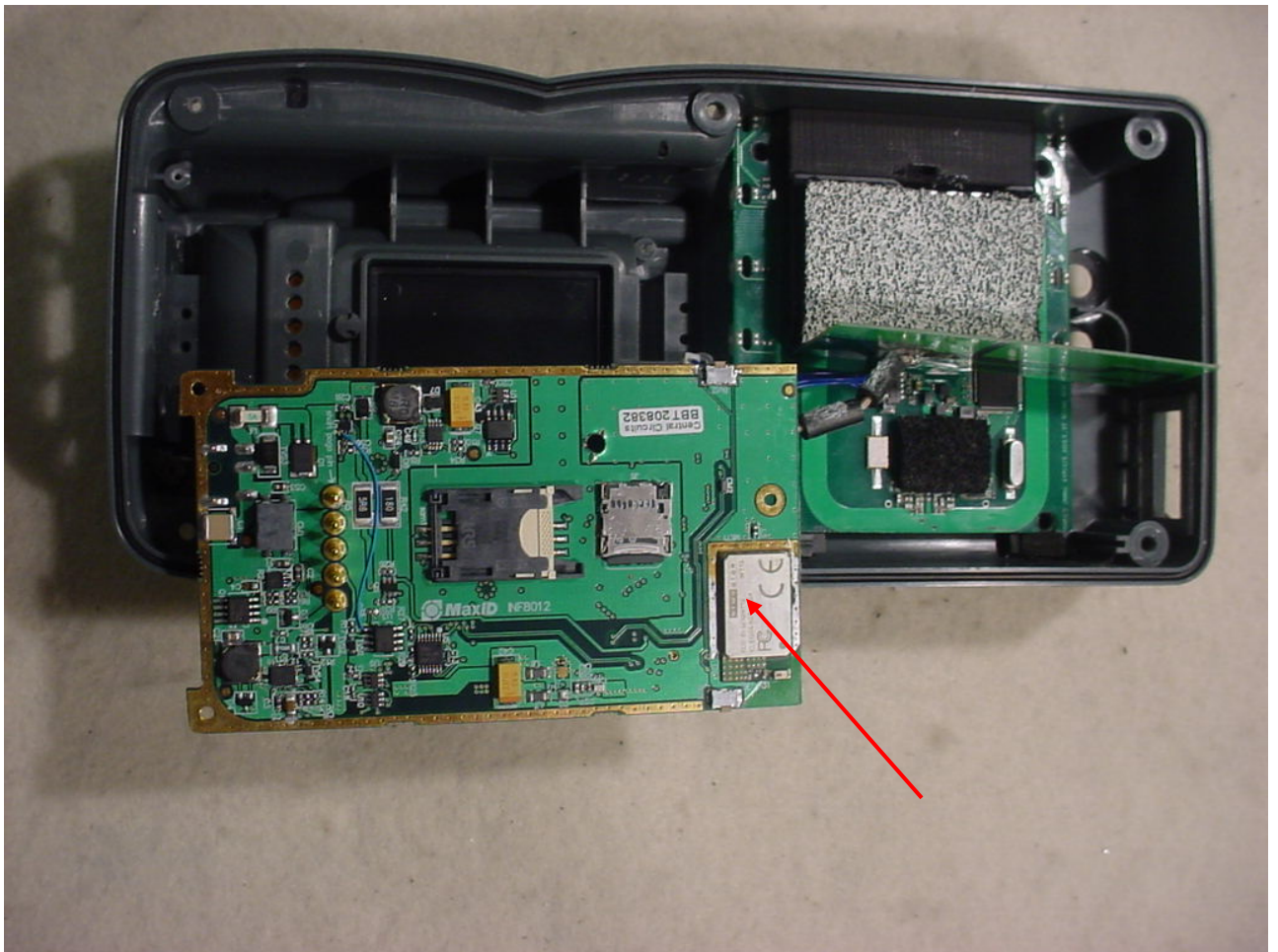
Figure 4: Bluetooth Module Placement
