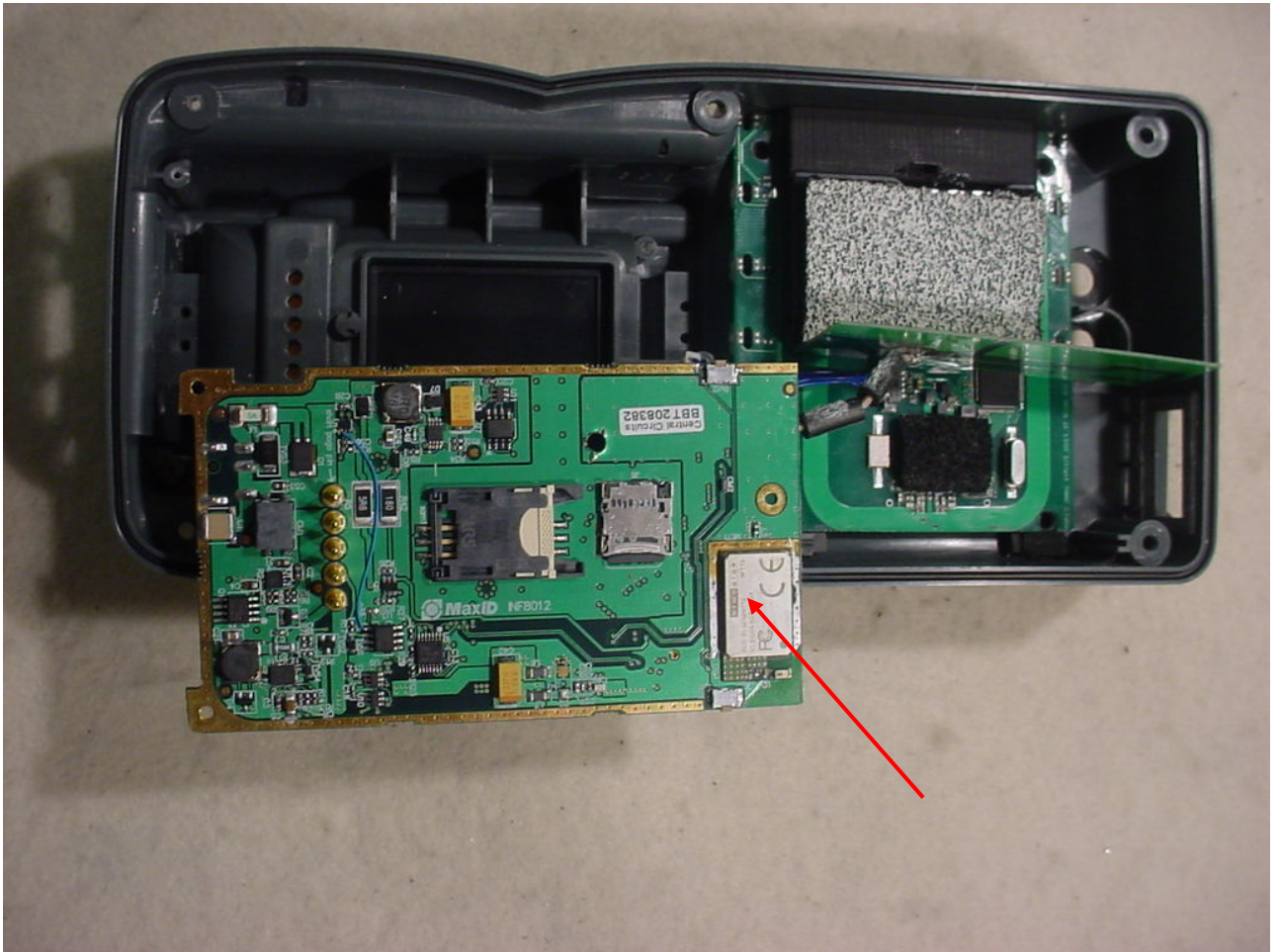
Figure 6: Bluetooth Module Placement
