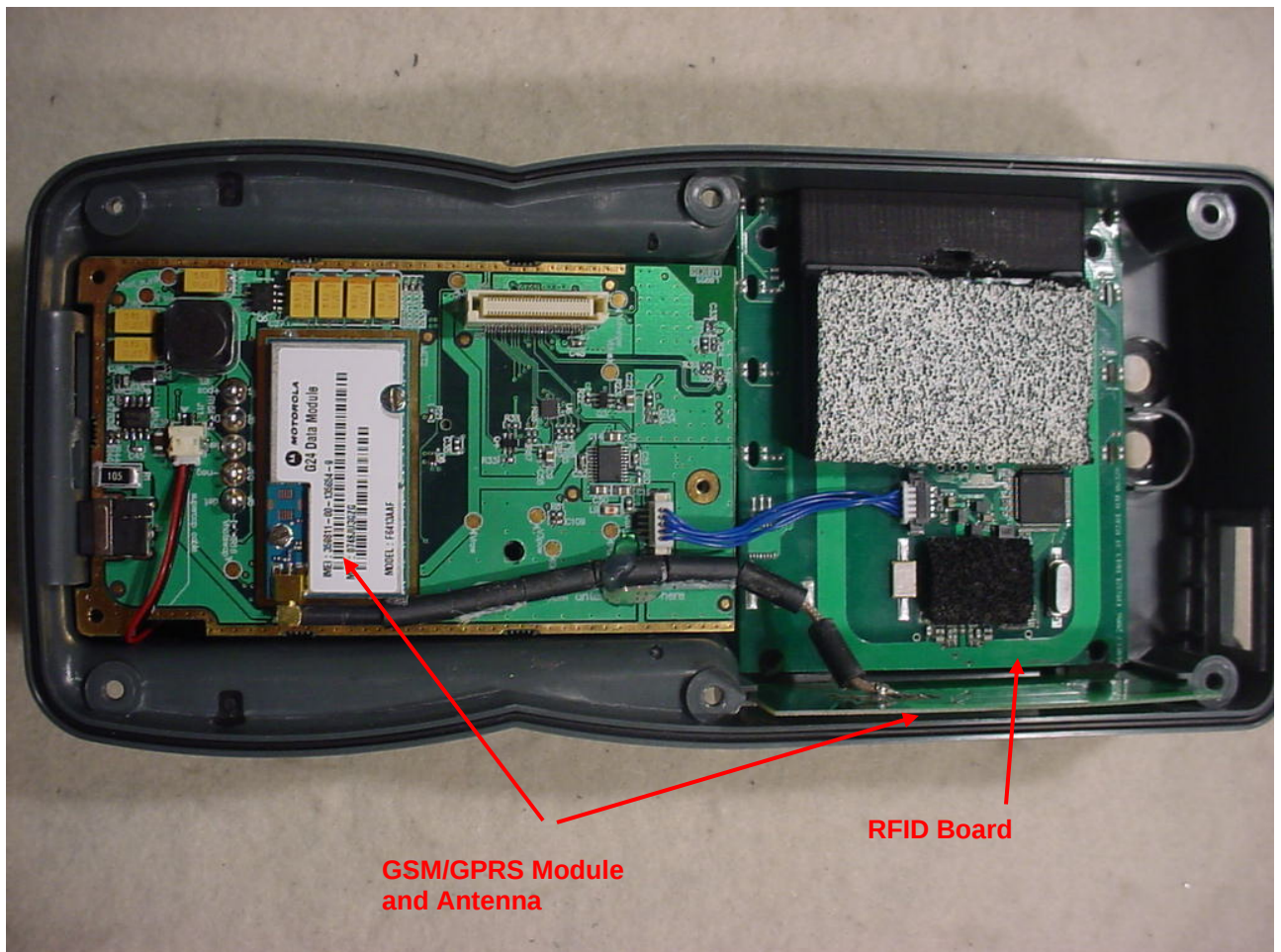
Figure 5: RFID Board and GSM/GPRS Module Placement and Antenna
