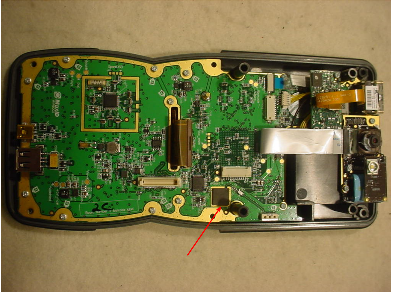
Figure 4: 802.11 Module Placement
