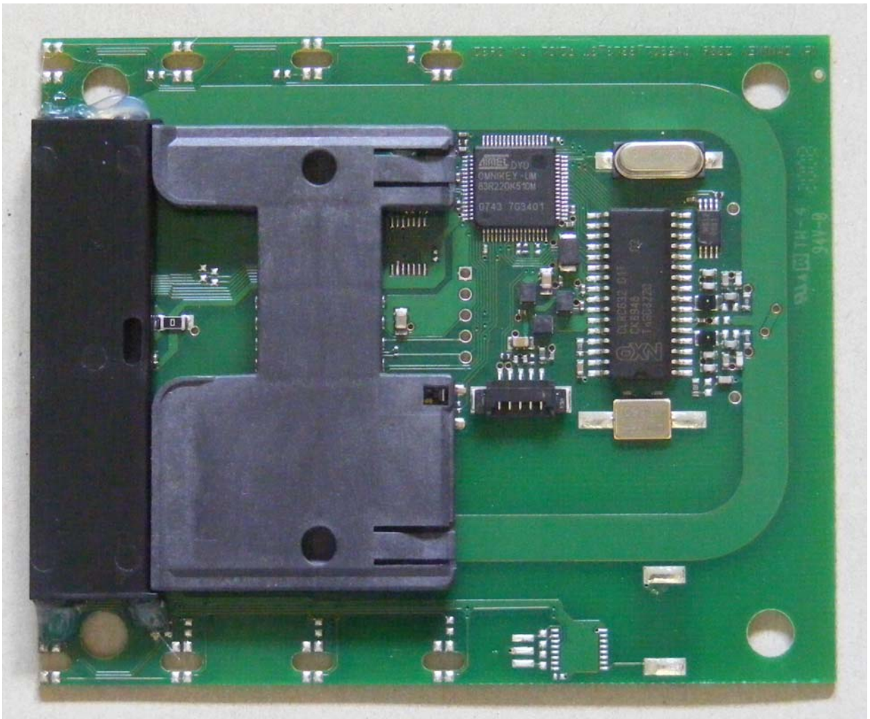
Figure 2: RFID Board Front
