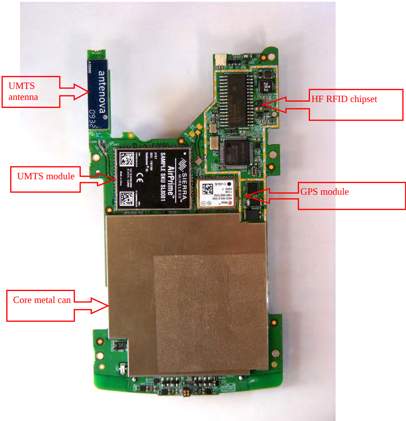
Main board top view
