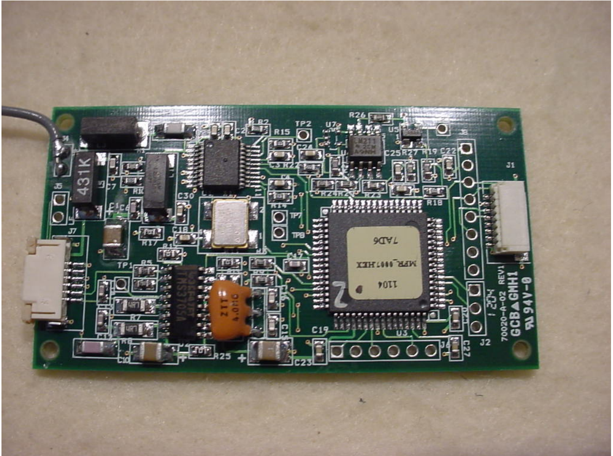
Figure 4: Top View of 13.5MHz RF Board
