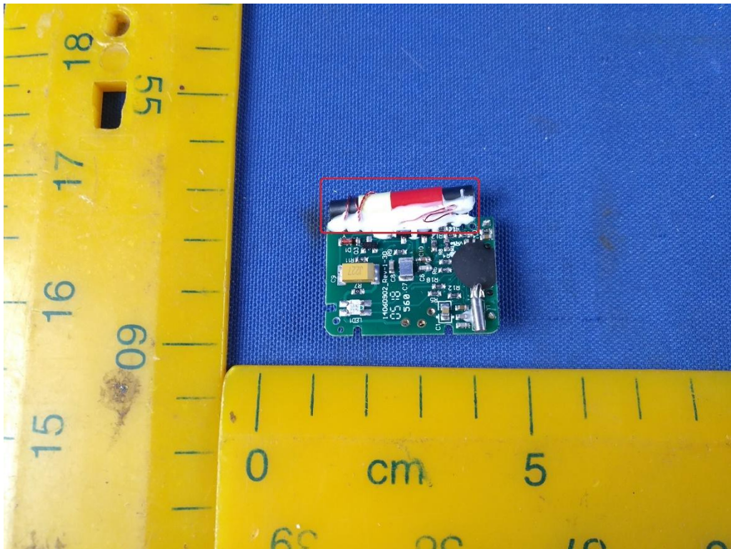
Antenna Position
