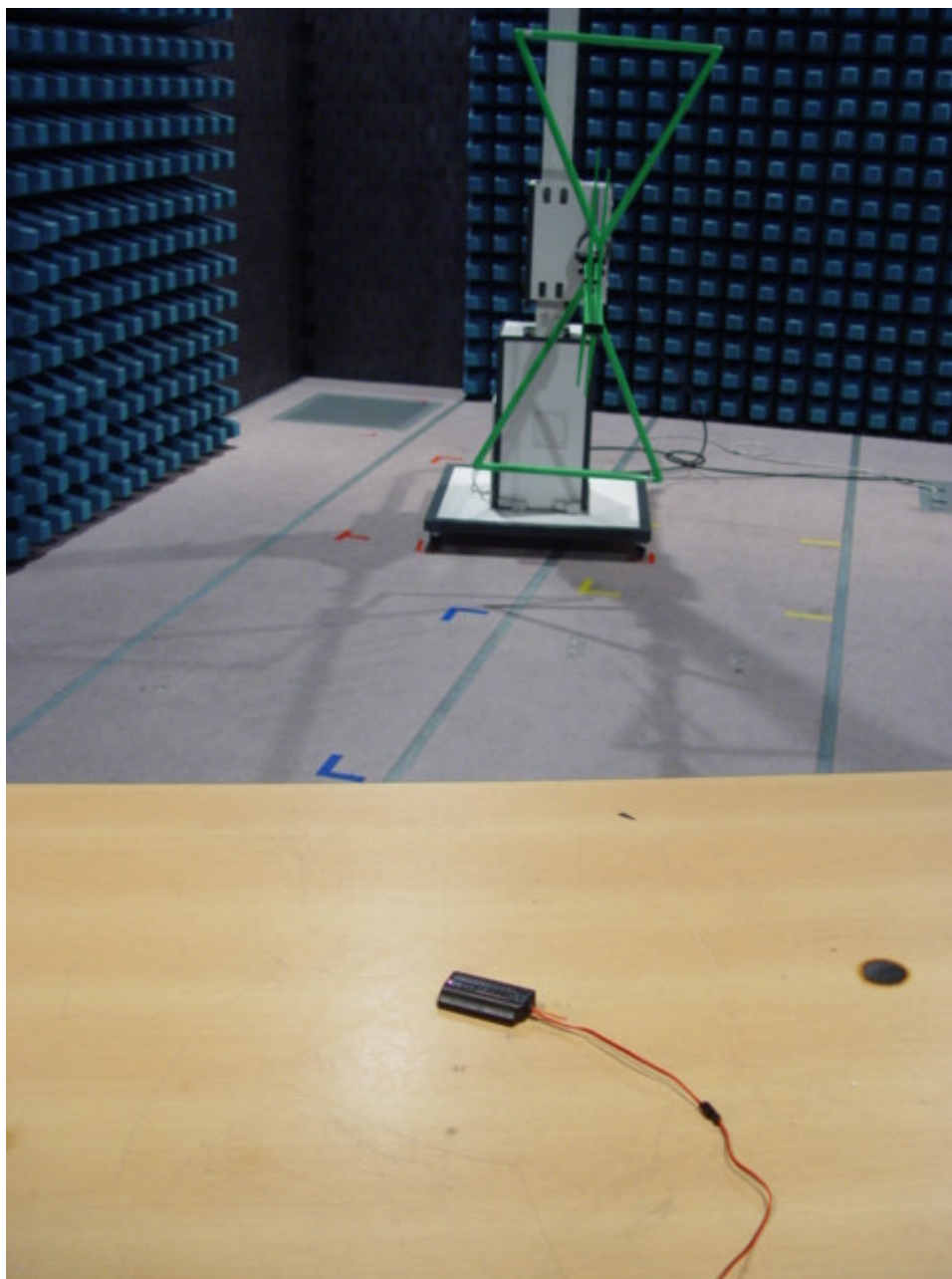
Photograph 1: Set-up for Radiation Measurement Below 1GHz
