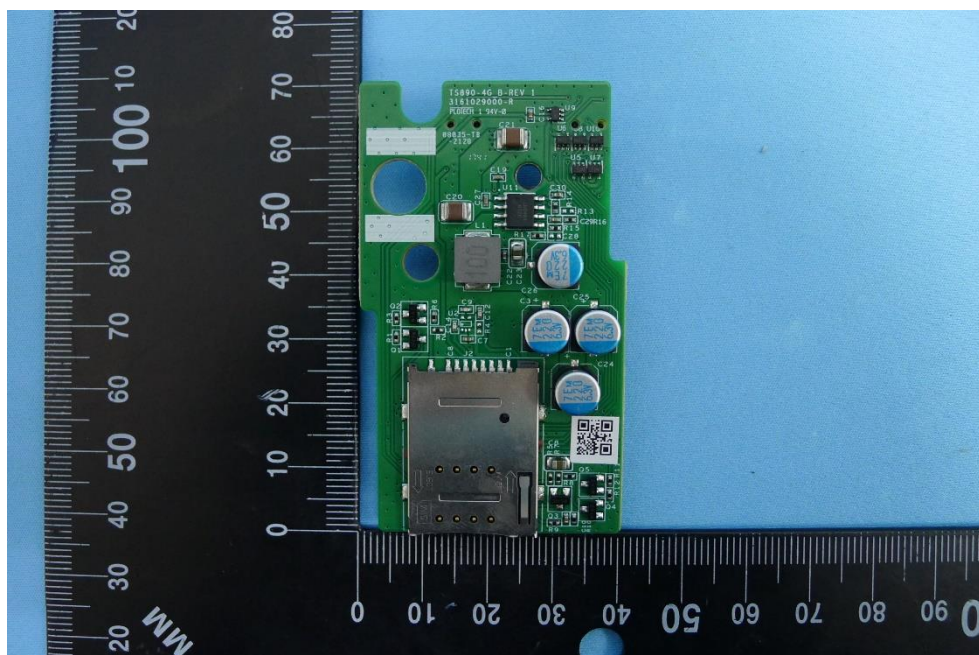
(32) EUT Photo (TS890G without Battery)
