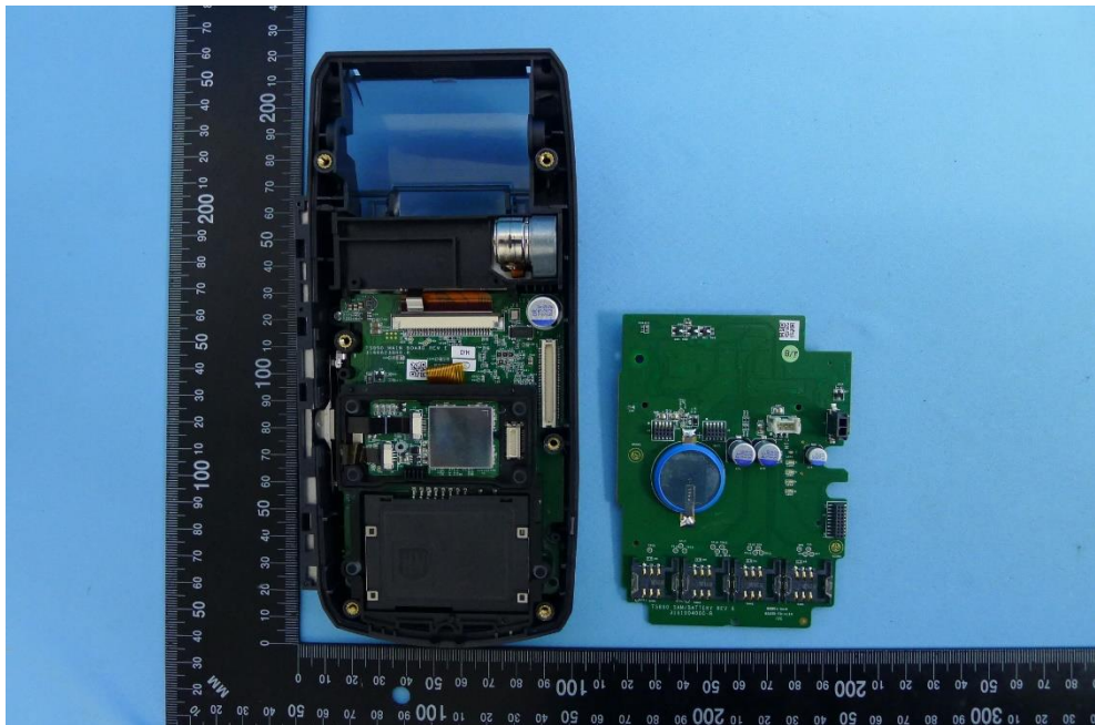
(12) EUT Photo (TS890G with Battery(Optional))
