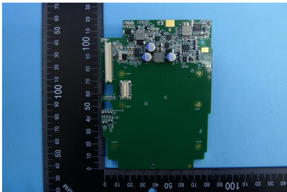
(14) EUT Photo (TS890G with Battery(Optional))
