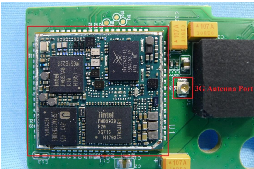
(34) EUT Photo (TS890G without Battery)
