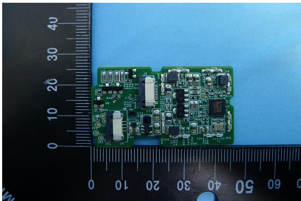
(20) EUT Photo (TS890G with Battery(Optional))
