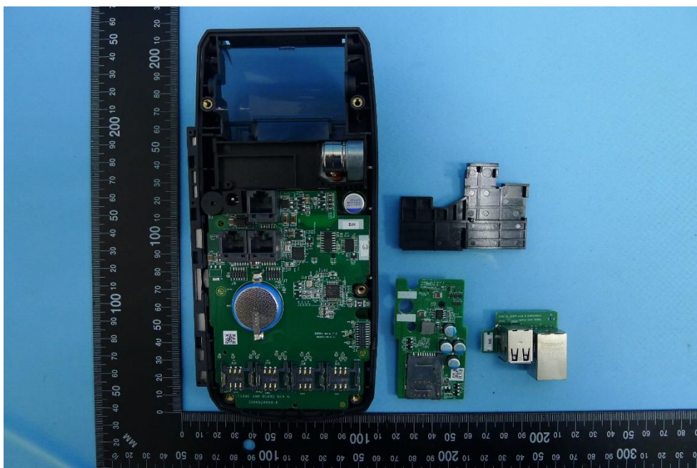
(28) EUT Photo (TS890G without Battery)
