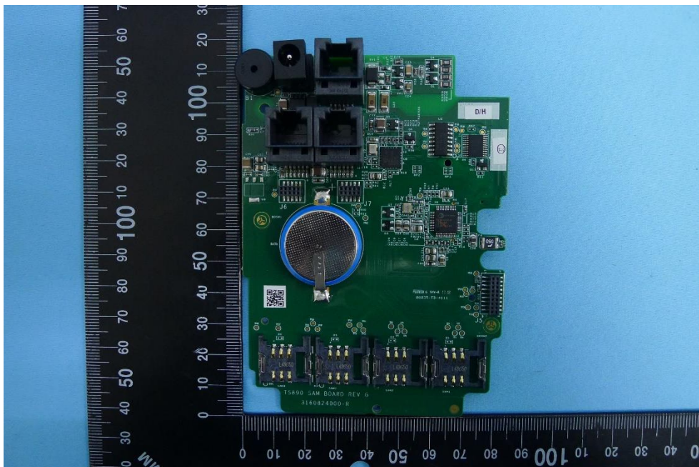
(36) EUT Photo (TS890G without Battery)
