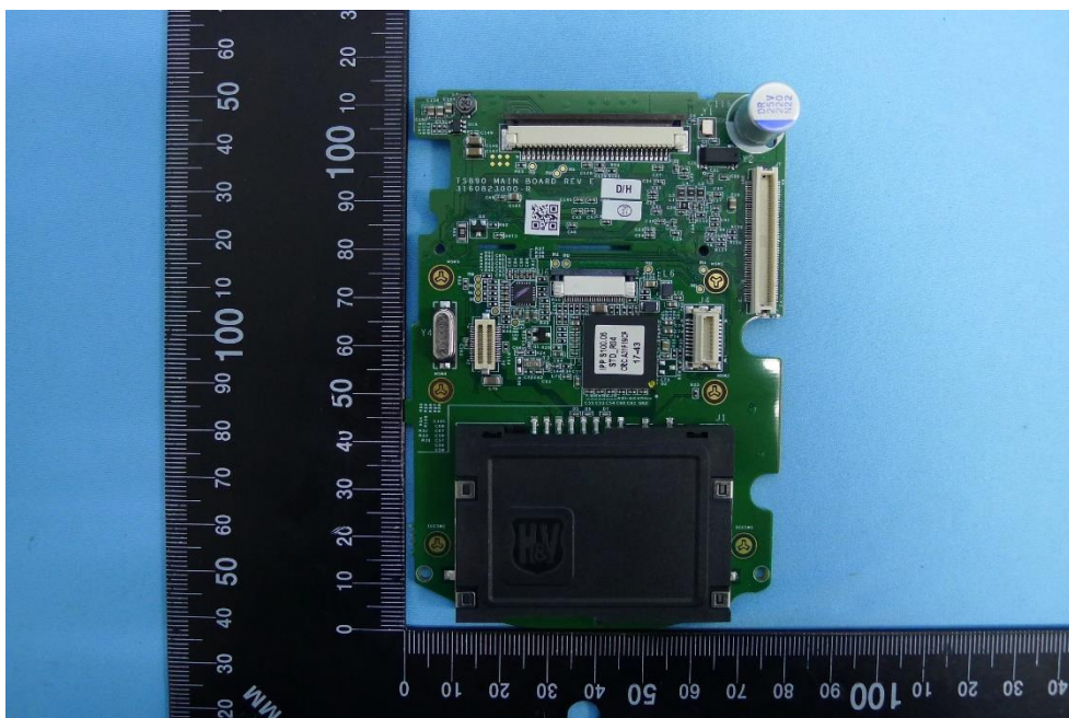
(16) EUT Photo (TS890G with Battery(Optional))
