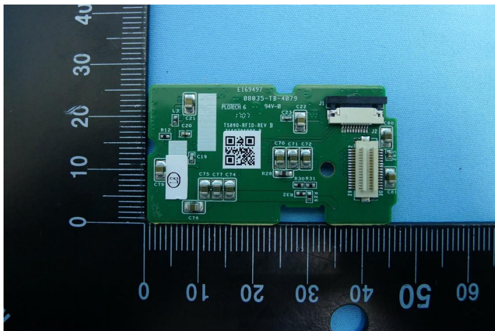
(44) EUT Photo (TS890G without Battery)
