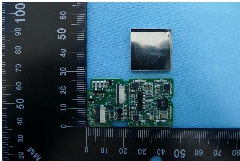
(42) EUT Photo (TS890G without Battery)
