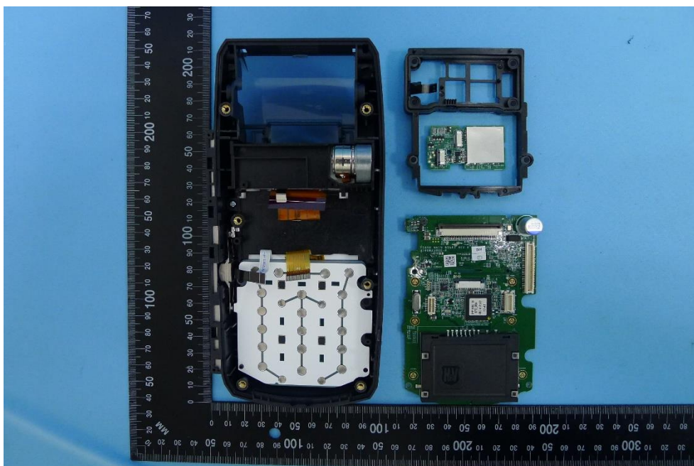
(38) EUT Photo (TS890G without Battery)
