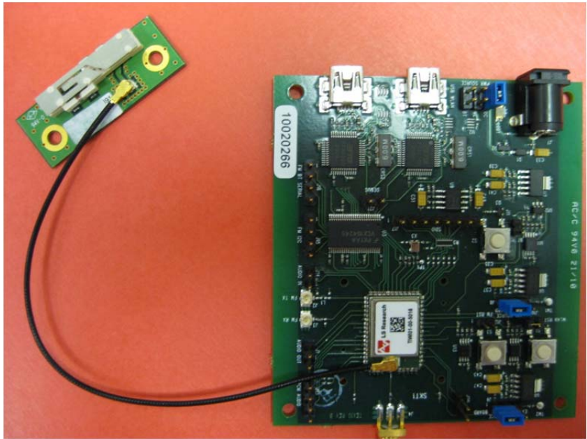
Module with embedded antenna connected
