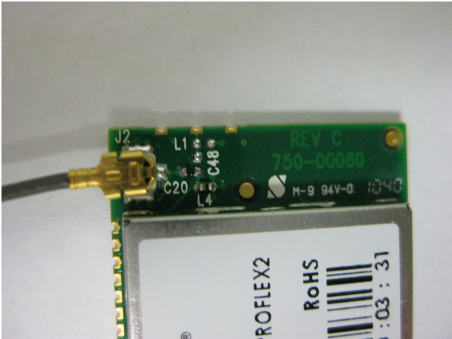
Antenna Connection Board Side
