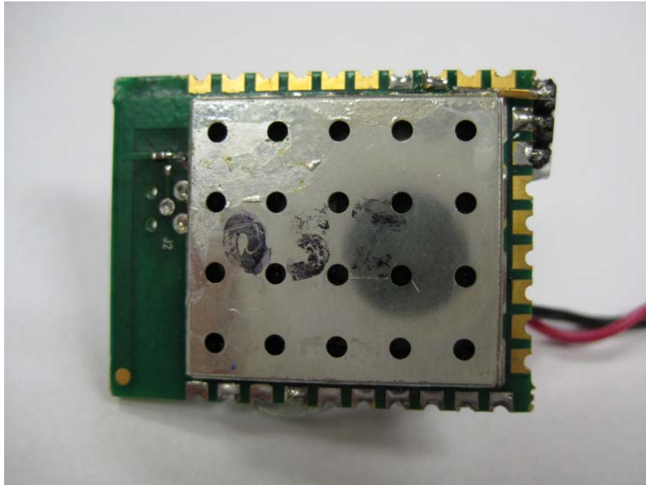
Front View 1 – Shielded (PCB Trace Antenna)
