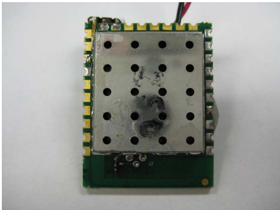
Front View 2 – Shielded (PCB Trace Antenna)
