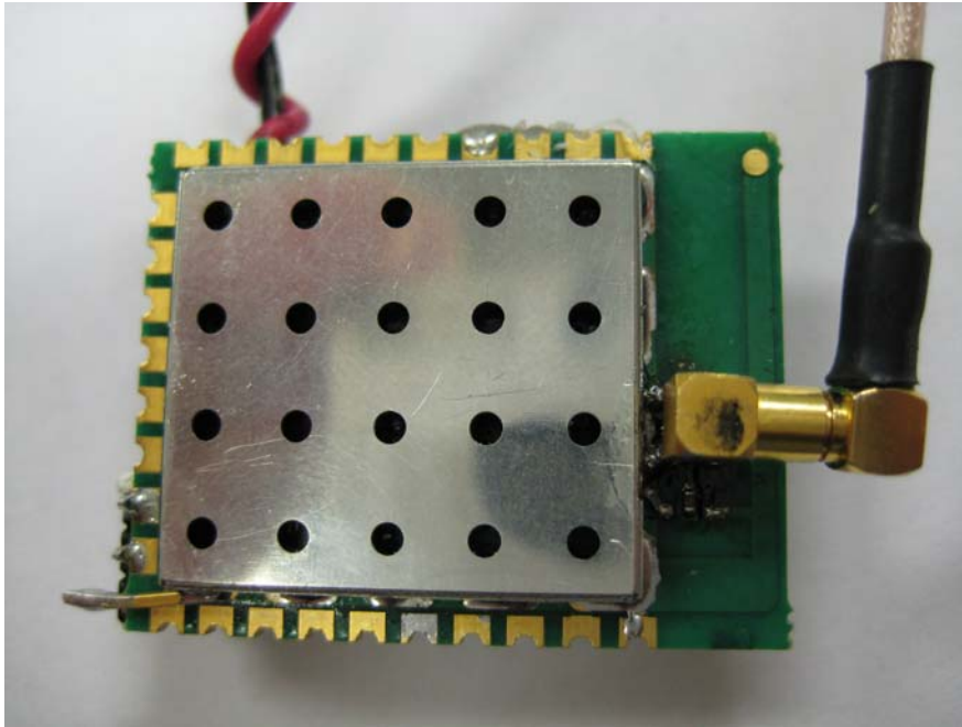
Front View 1 – Shielded (DiPole Antenna) Showing Antenna Connected
