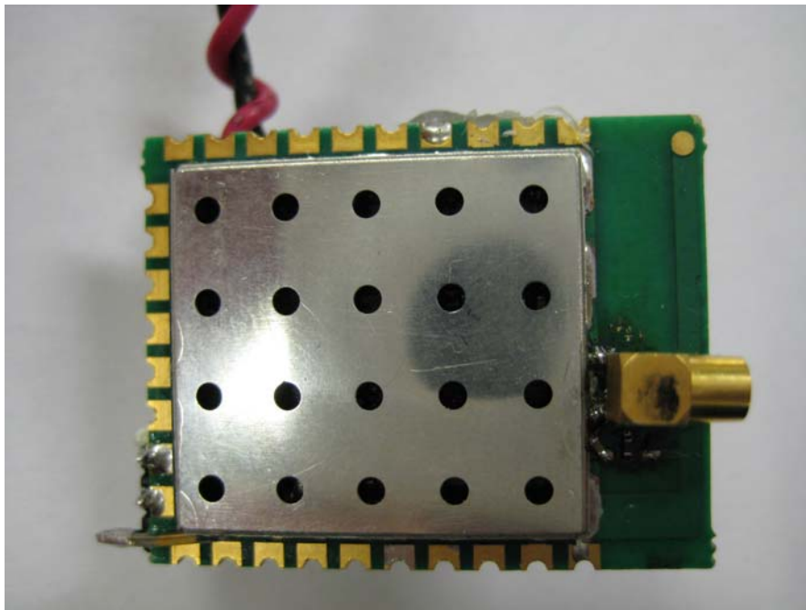
Front View 2 – Shielded (DiPole Antenna) Showing Antenna Connector
