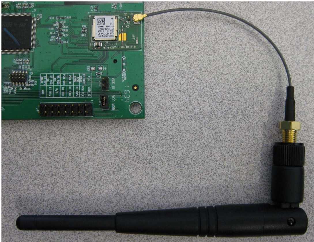
2.4/5.5 GHz Dipole Antenna with Reverse Polarity SMA Connector (001-0009)
