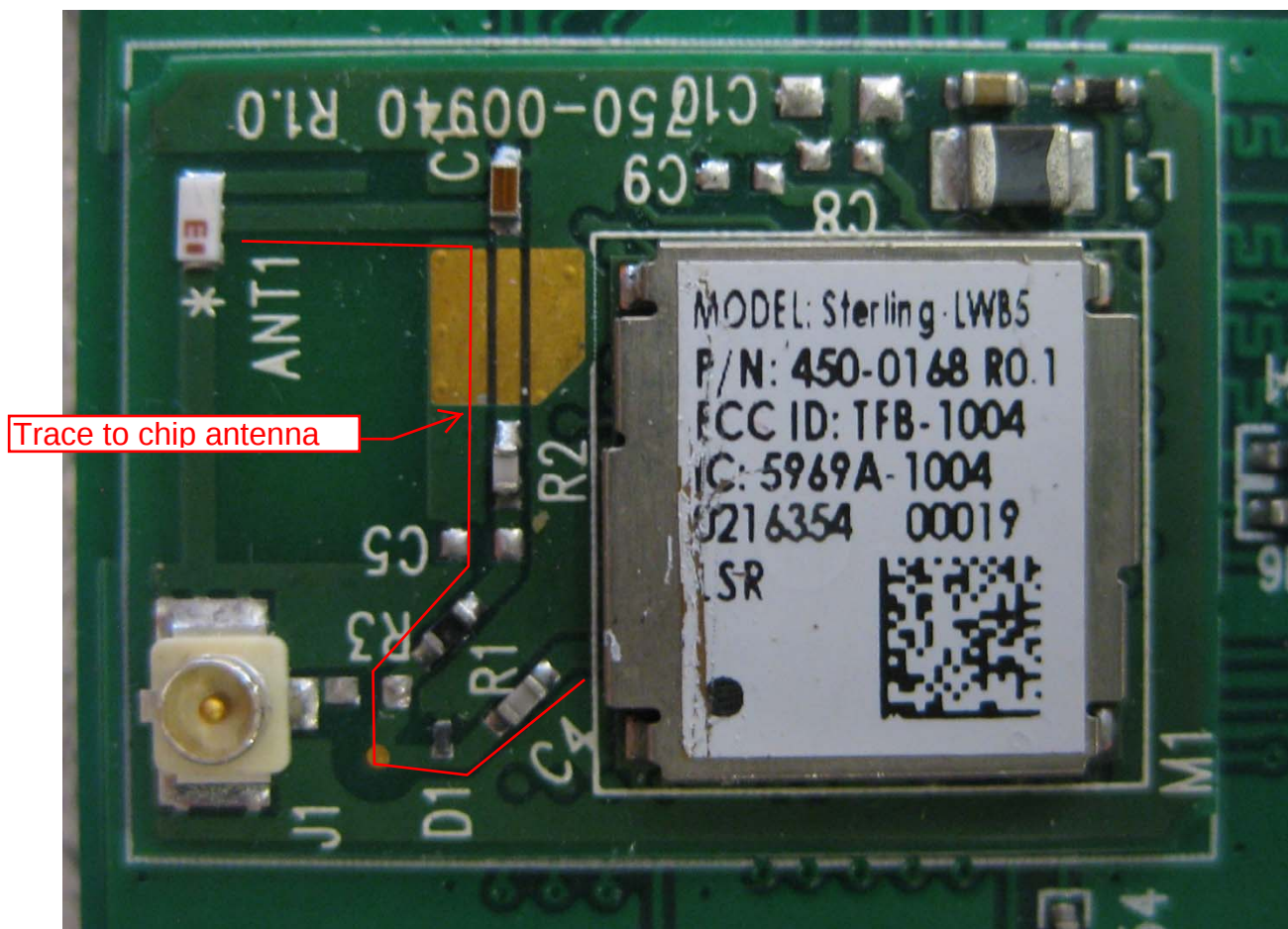
Module with Chip Antenna
