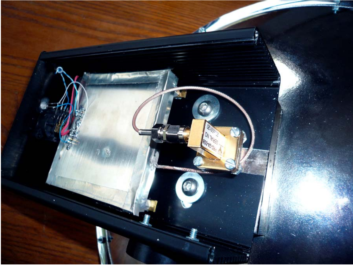
Transmitter with Parabolic antenna (2 photos):
