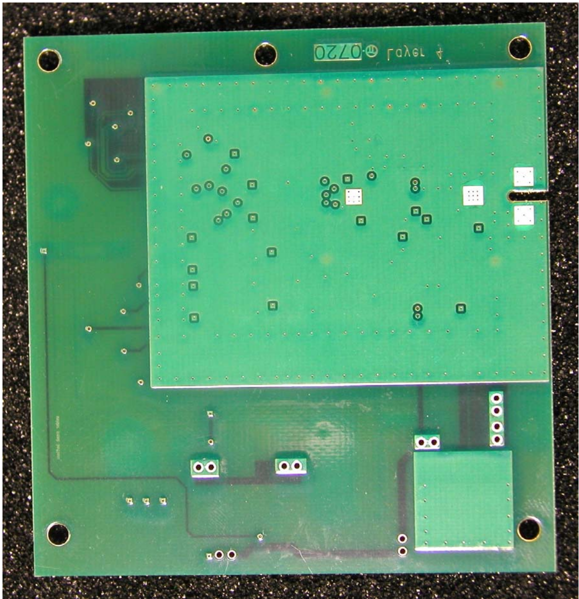
Transmitter Printed Circuit Board, bottom
