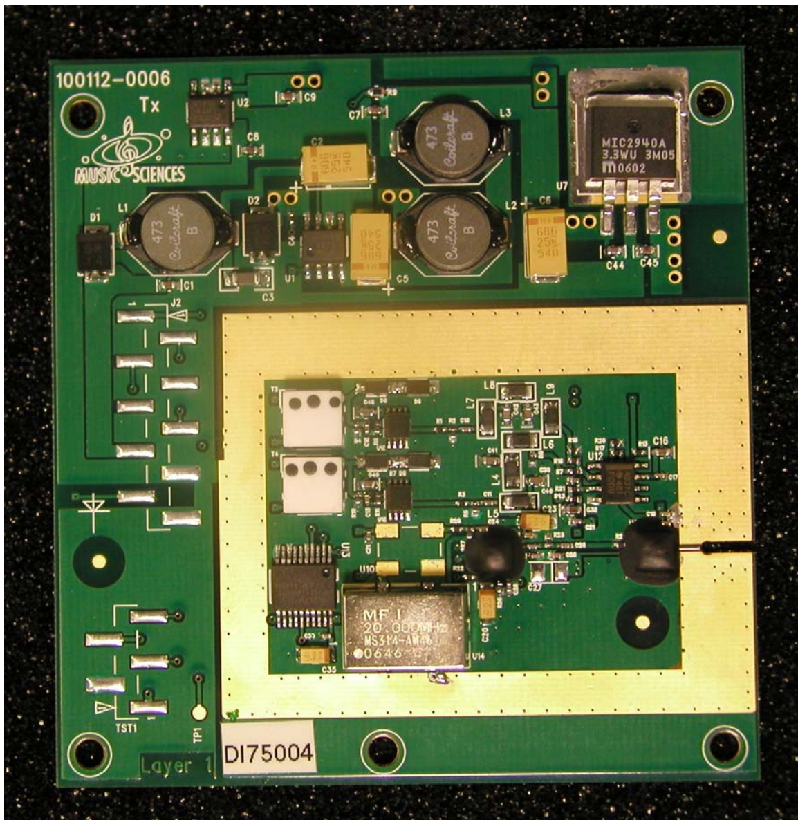
Transmitter Printed Circuit Board, top
