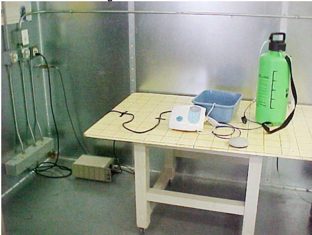
View of the EUT during the conducted emissions onto AC mains.
