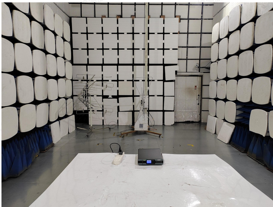
Radiated Emissions Measurement (Below 1GHz)
