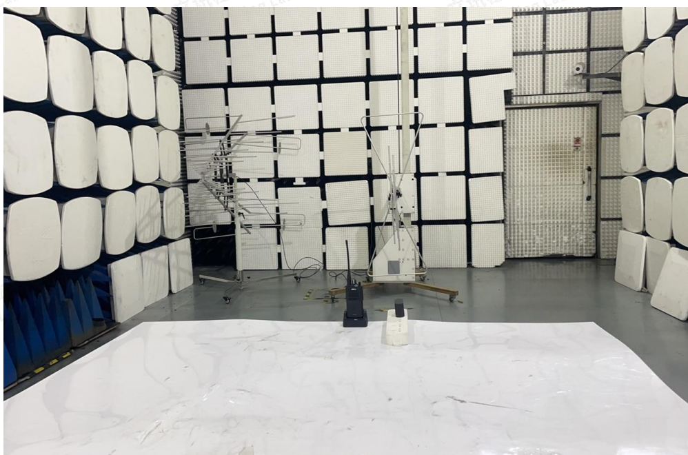
Radiated Emissions Measurement (Below 1GHz)
