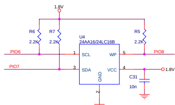
Serial EEPROM
