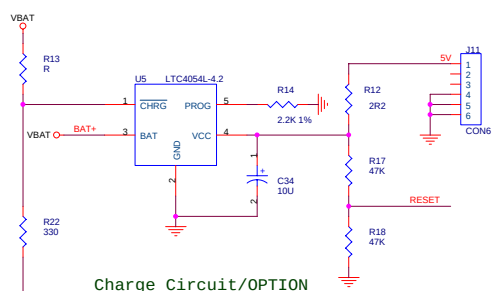
Charge Circuit/OPTION
