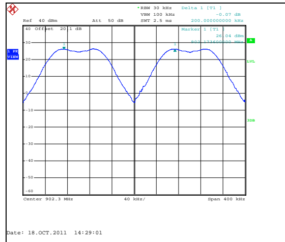
Figure 7.4.1.2-1: 50kbps Data Rate (SUN Mode)
