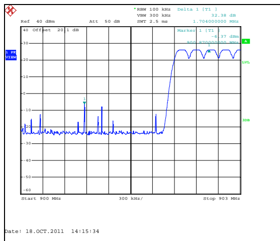
Figure 7.5.1.2-3: Lower Band-edge
