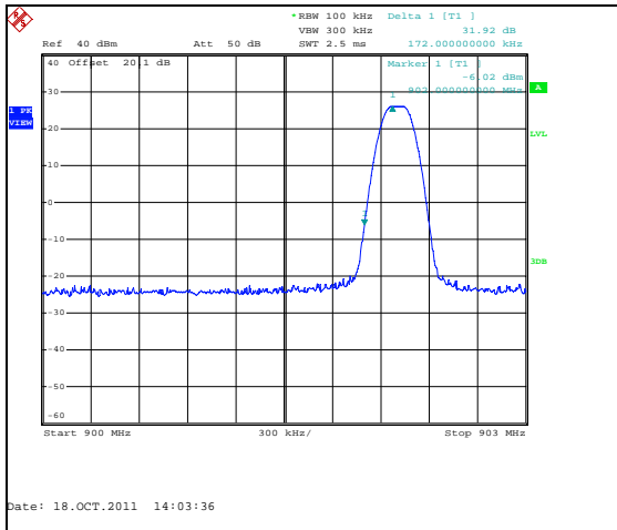
Figure 7.5.1.2-1: Lower Band-edge
