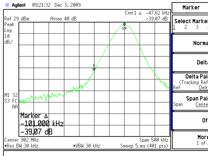
Figure 6.8.1-1: Lower Band-Edge (9600 BPS)
