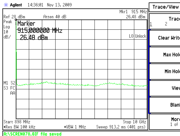
Figure 6.8.2-4: RF Conducted Spurious Emissions – Mid Channel
