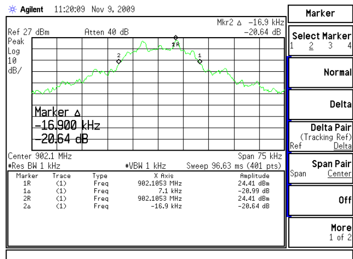
Figure 6.7.4-1: 20dB Bandwidth – Low Channel (9600 BPS)
