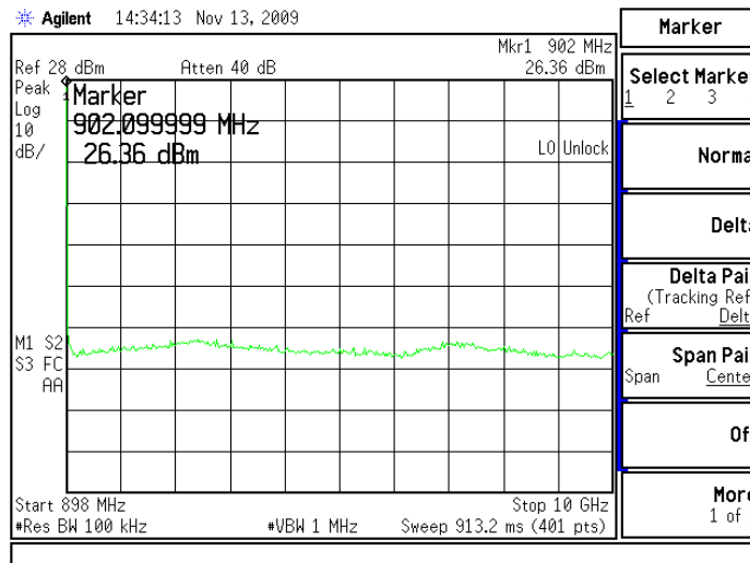
Figure 6.8.2-2: RF Conducted Spurious Emissions – Low Channel
