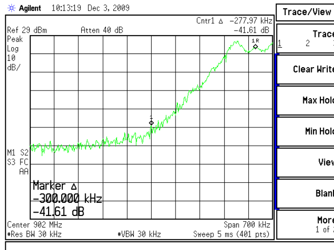
Figure 6.8.1-9: Lower Band-Edge (115200 BPS)
