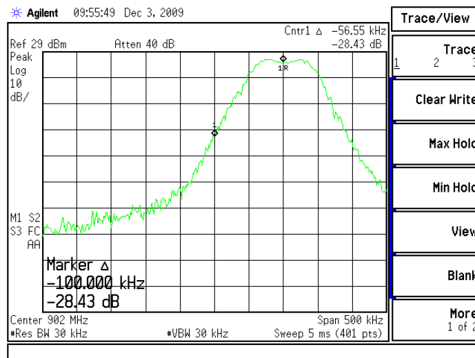
Figure 6.8.1-5: Lower Band-Edge (38400 BPS)
