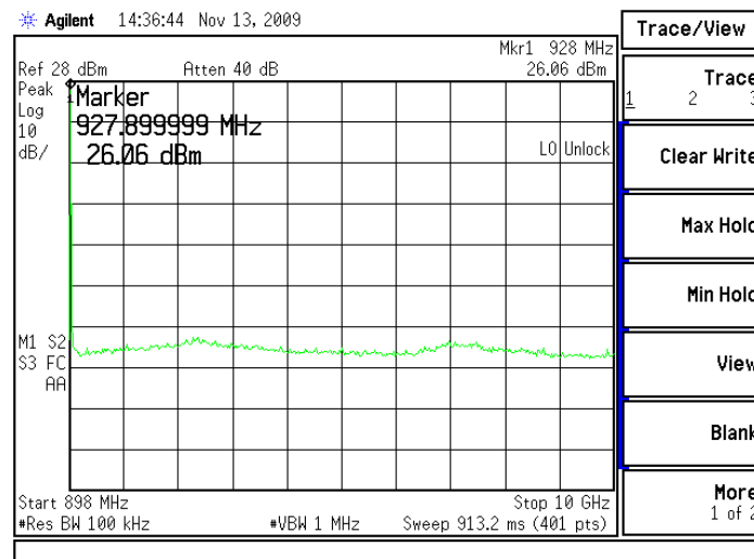
Figure 6.8.2-6: RF Conducted Spurious Emissions – High Channel
