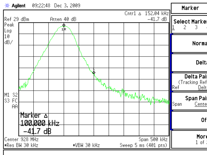
Figure 6.8.1-2: Upper Band-Edge (9600 BPS)
