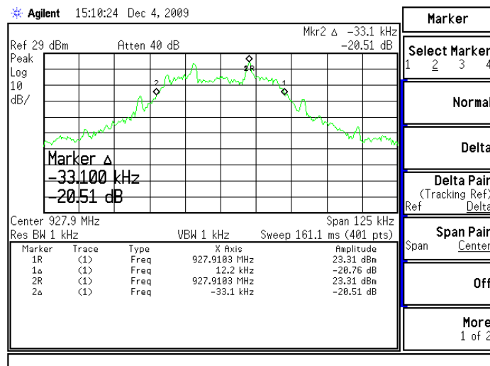
Figure 6.7.4-6: 20dB Bandwidth – High Channel (19200 BPS)
