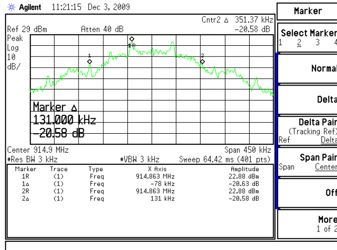
Figure 6.7.4-11: 20dB Bandwidth – Mid Channel (76800 BPS)
