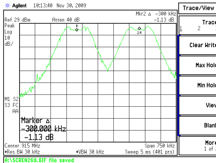
Figure 6.7.1-2: Carrier Frequency Separation 76.8 and 115.2 Kbps
