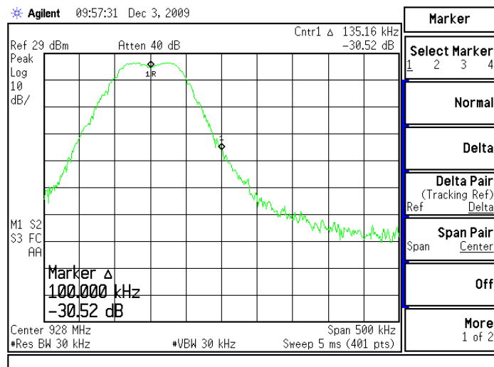
Figure 6.8.1-6: Upper Band-Edge (38400 BPS)
