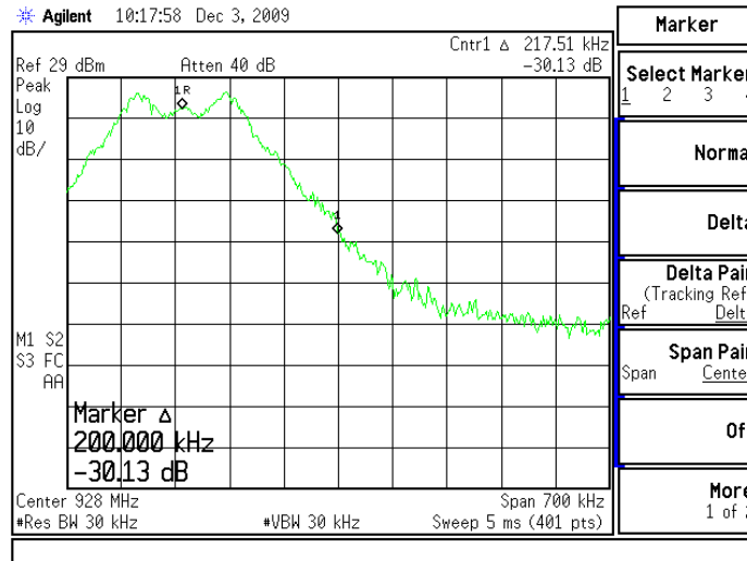
Figure 6.8.1-10: Upper Band-Edge (115200 BPS)
