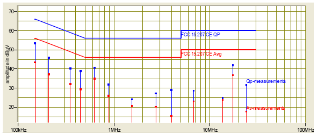
Figure 6.4-1: Power Line Conducted Emissions Summary
