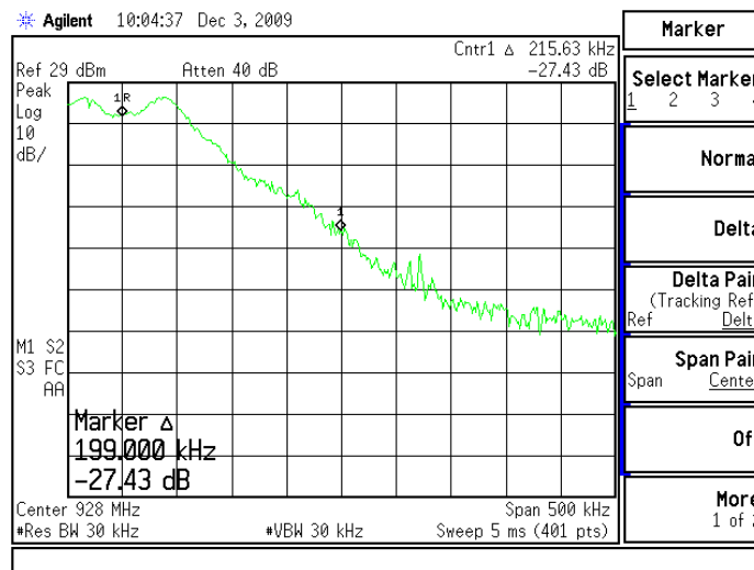
Figure 6.8.1-8: Upper Band-Edge (76800 BPS)
