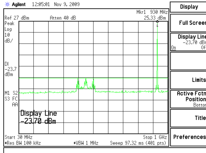
Figure 6.8.2-5: RF Conducted Spurious Emissions – High Channel
