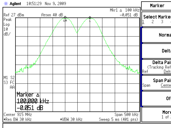
Figure 6.7.1-1: Carrier Frequency Separation \leq 38.4 Kbps
