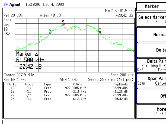
Figure 6.7.4-9: 20dB Bandwidth – High Channel (38400 BPS)
