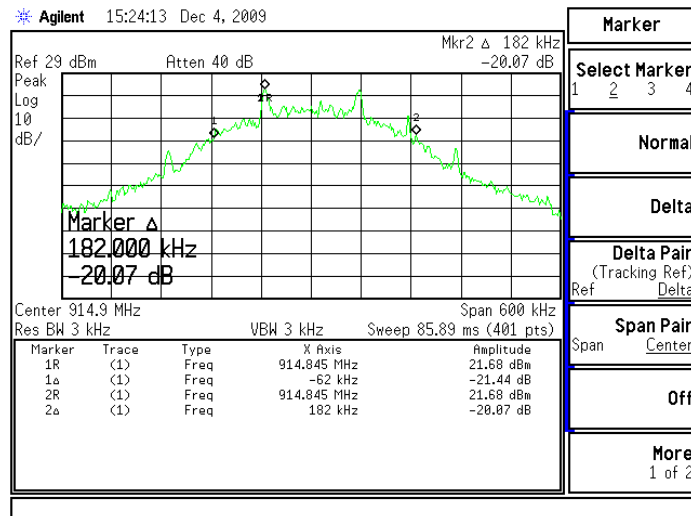
Figure 6.7.4-14: 20dB Bandwidth – Mid Channel (115200 BPS)
