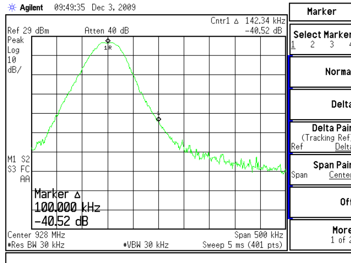
Figure 6.8.1-4: Upper Band-Edge (19200 BPS)
