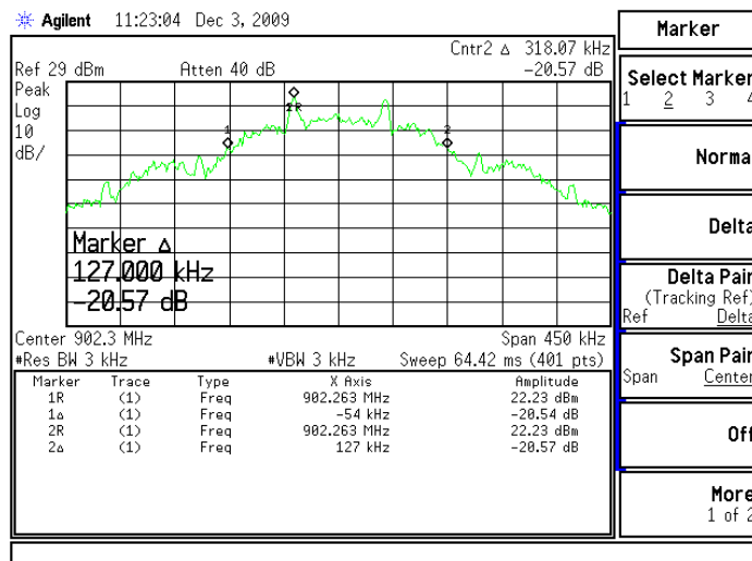
Figure 6.7.4-10 20dB Bandwidth – Low Channel (76800 BPS)
