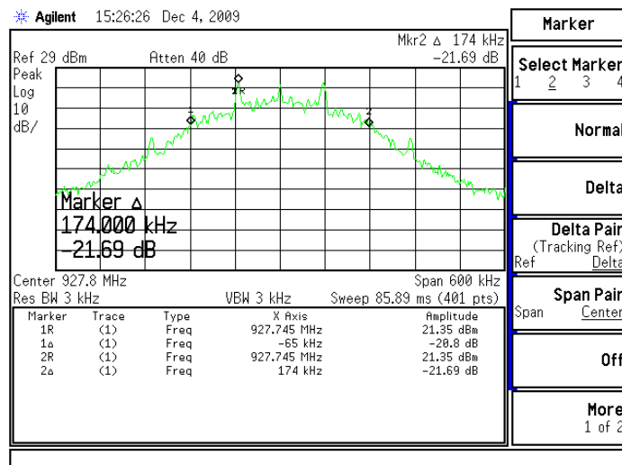
Figure 6.7.4-15: 20dB Bandwidth – High Channel (115200 BPS)
