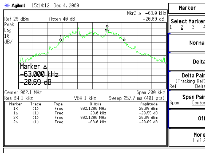
Figure 6.7.4-7: 20dB Bandwidth – Low Channel (38400 BPS)
