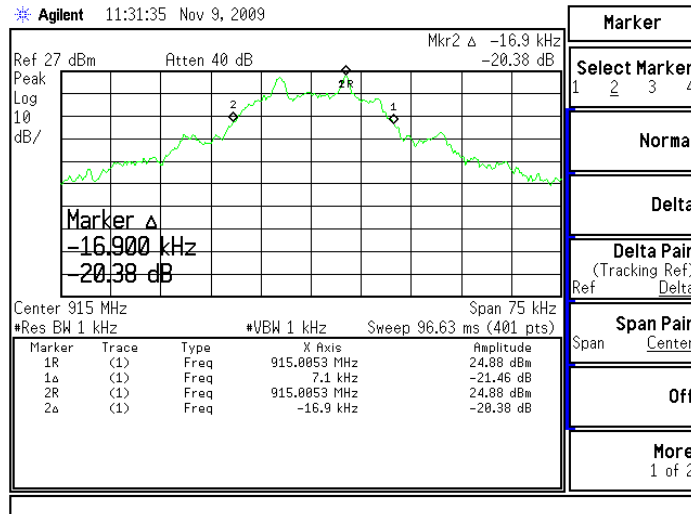
Figure 6.7.4-2: 20dB Bandwidth – Mid Channel (9600 BPS)
