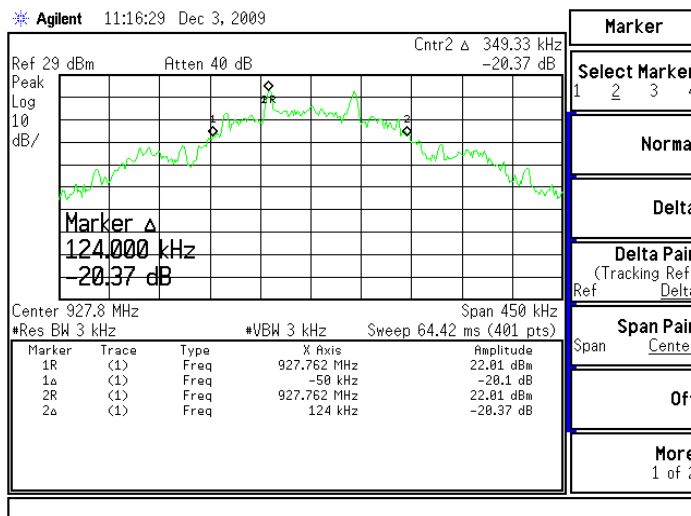
Figure 6.7.4-12: 20dB Bandwidth – High Channel (76800 BPS)
