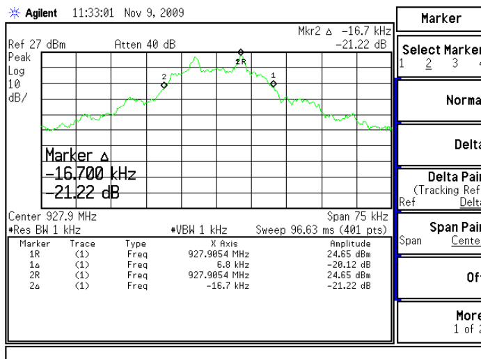
Figure 6.7.4-3: 20dB Bandwidth – High Channel (9600 BPS)
