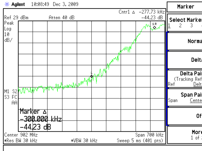
Figure 6.8.1-7: Lower Band-Edge (76800 BPS)
