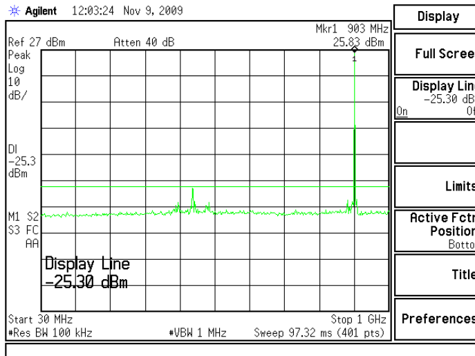
Figure 6.8.2-1: RF Conducted Spurious Emissions – Low Channel
