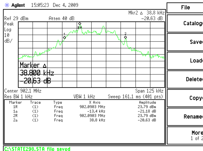
Figure 6.7.4-4: 20dB Bandwidth – Low Channel (19200 BPS)
