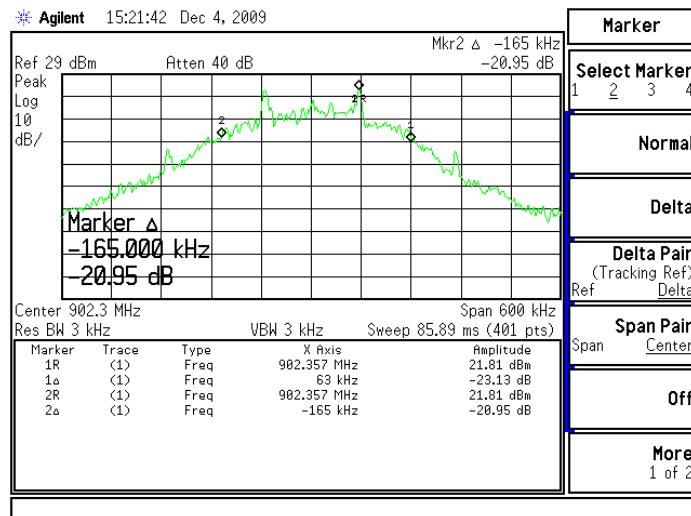
Figure 6.7.4-13: 20dB Bandwidth – Low Channel (115200 BPS)
