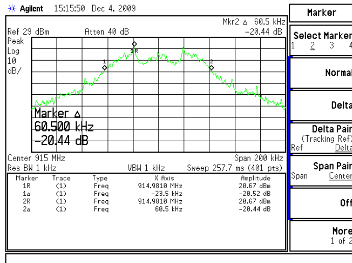
Figure 6.7.4-8: 20dB Bandwidth – Mid Channel (38400 BPS)
