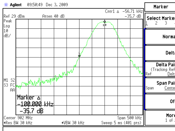
Figure 6.8.1-3: Lower Band-Edge (19200 BPS)
