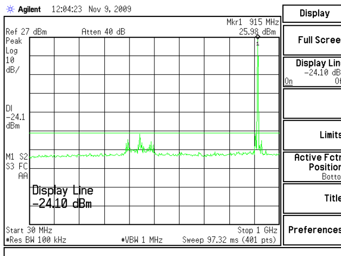
Figure 6.8.2-3: RF Conducted Spurious Emissions – Mid Channel
