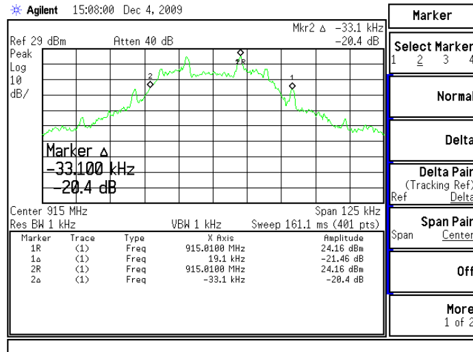
Figure 6.7.4-5: 20dB Bandwidth – Mid Channel (19200 BPS)
