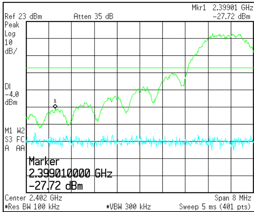
Figure 6.9-1: Lower Band-Edge (Conducted)
