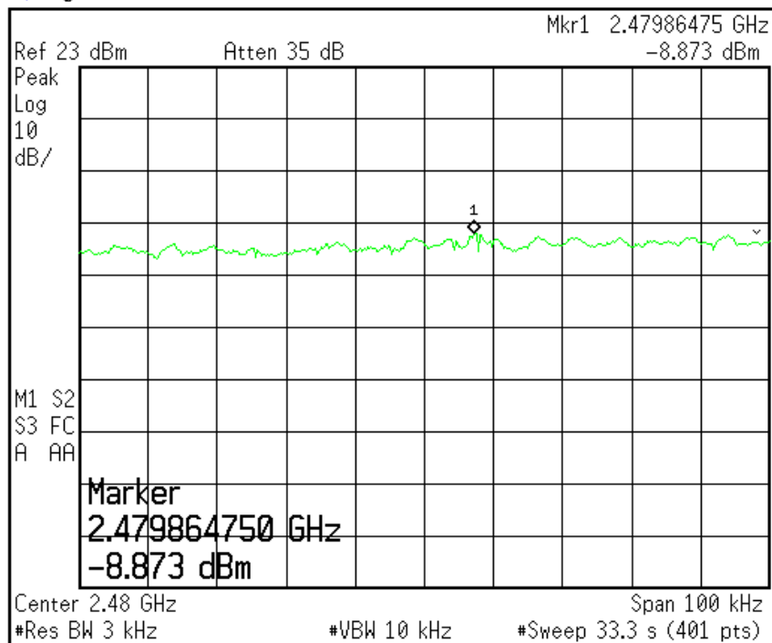
Figure 6.8-3: Power Spectral Density Plot – High Channel
