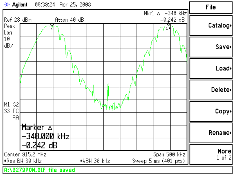
Figure 6.7.1-1: System One Carrier Frequency Separation
