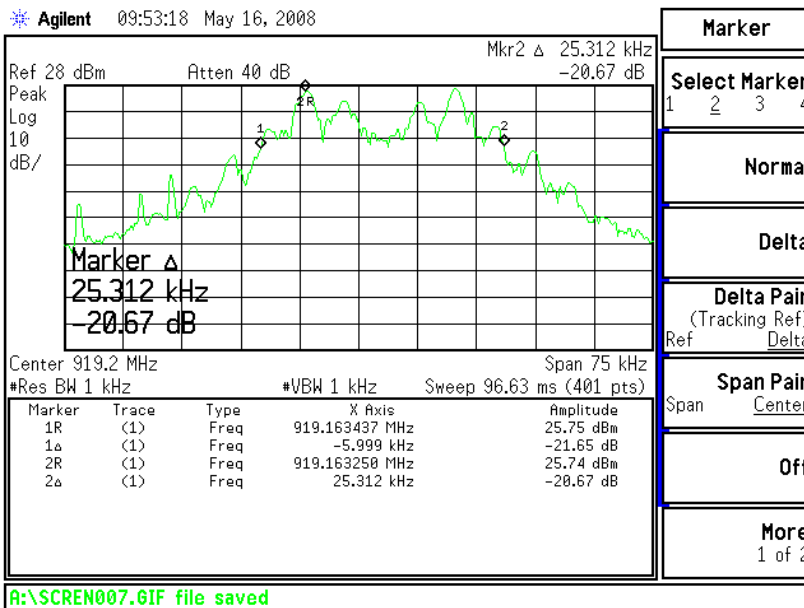
Figure 6.7.4-2: System One 20dB Bandwidth – Mid Channel
