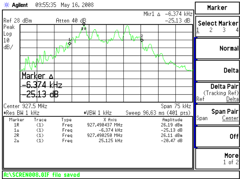
Figure 6.7.4-3: System One 20dB Bandwidth – High Channel
