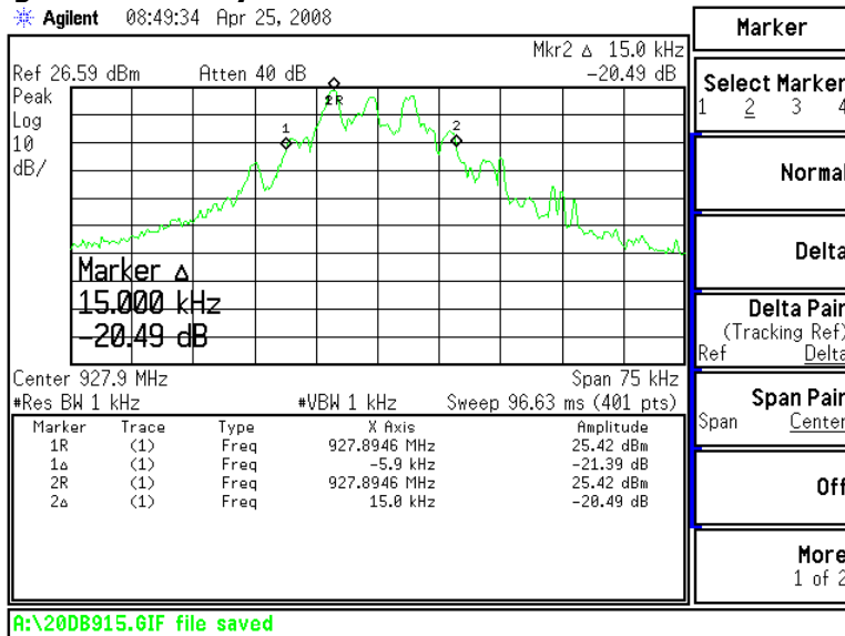
Figure 6.7.4-5: System Two 20dB Bandwidth – Mid Channel
