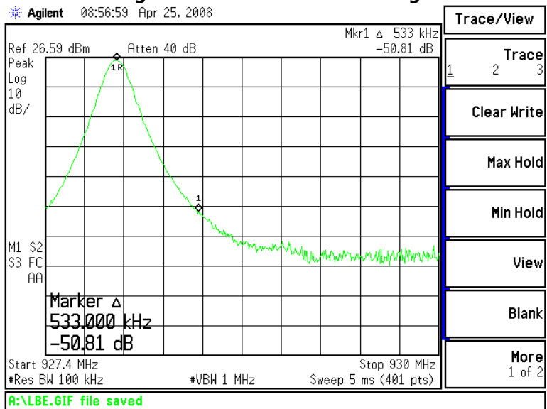
Figure 6.8.1-1: Lower Band-Edge
