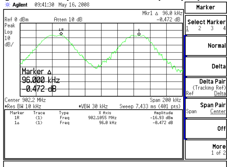
Figure 6.7.1-2: System Two Carrier Frequency Separation
