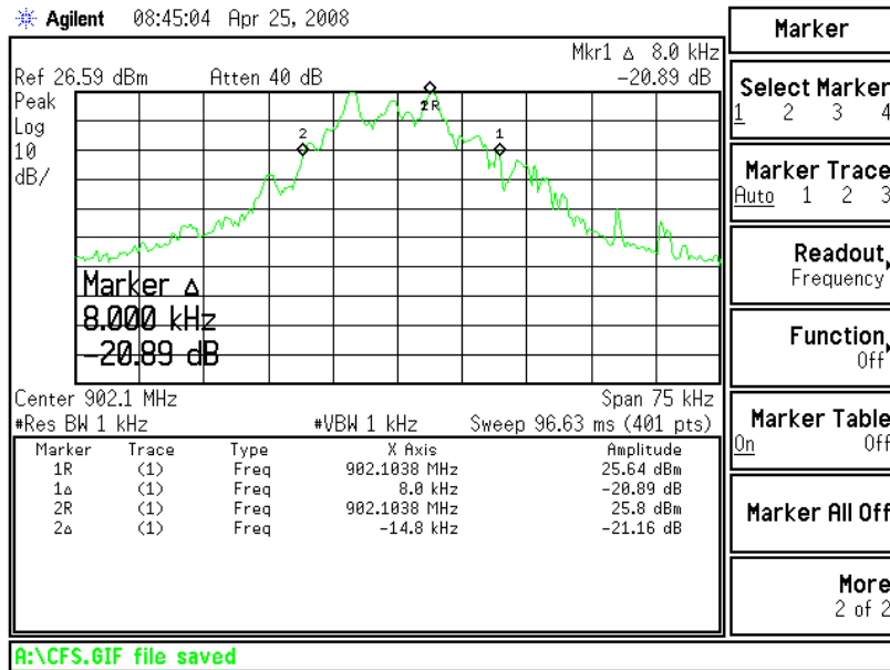
Figure 6.7.4-4: System Two 20dB Bandwidth – Low Channel
