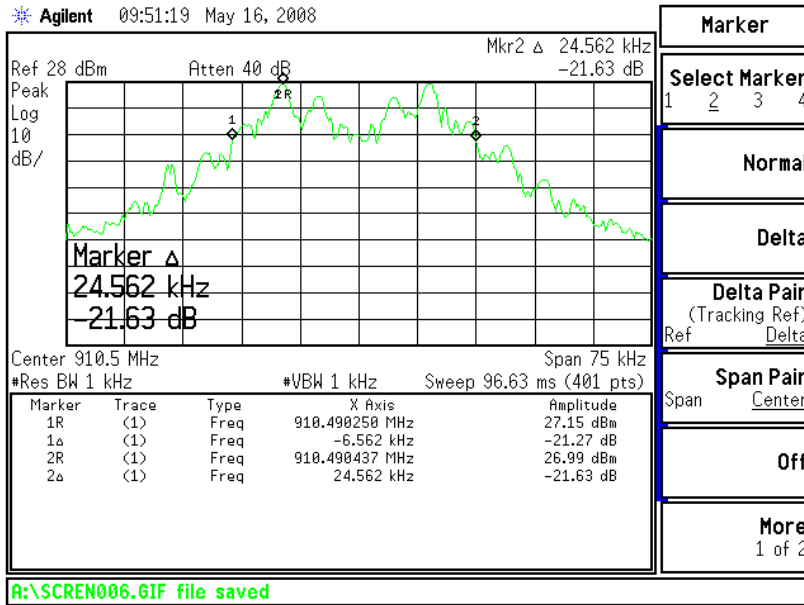
Figure 6.7.4-1: System One 20dB Bandwidth – Low Channel
