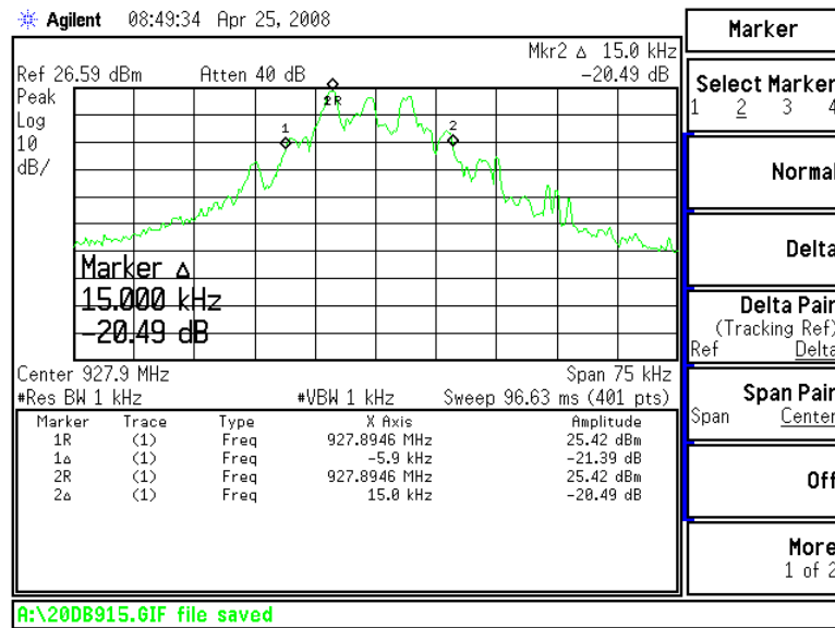
Figure 6.7.4-3: 20dB Bandwidth – High Channel
