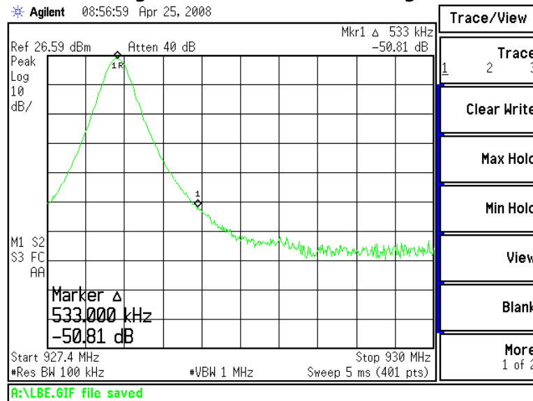
Figure 6.8.1-1: Lower Band-Edge
