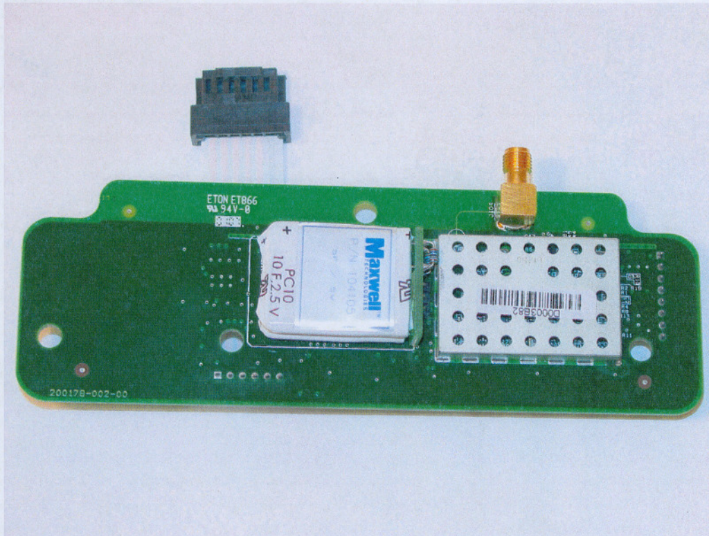
Back of S4 PCB:
