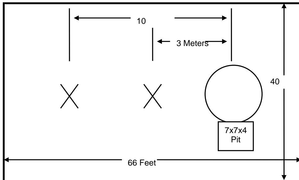
Figure 2.3.2-1: Open Area Test Site
