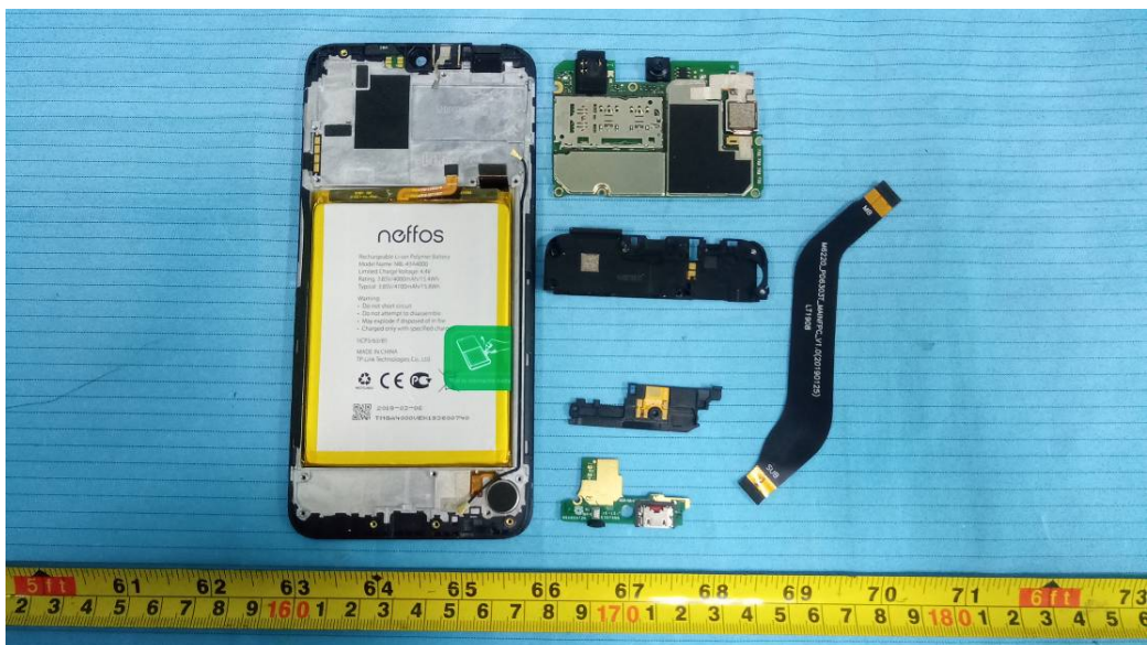
EUT – Cover off View 2
