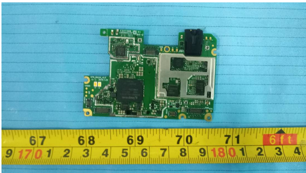
EUT – Main Board 1 Top Shielding off View
