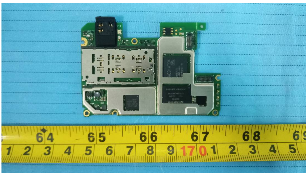
EUT – Main Board 1 Bottom Shielding off View
