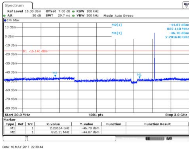
8-DPSK MIDDLE CHANNEL , SPURIOUS 30 MHz ~ 3 GHz
