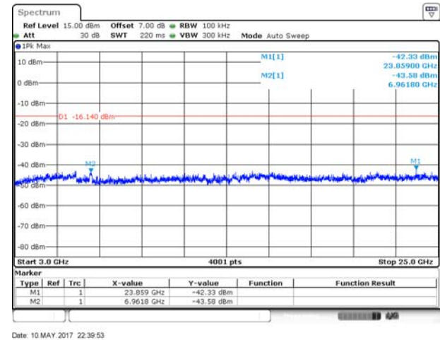
8-DPSK MIDDLE CHANNEL , SPURIOUS 3 GHz ~ 25 GHz
