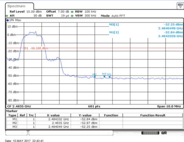
8-DPSK HIGH CHANNEL , BAND EDGE
