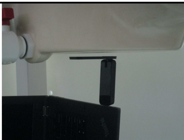
Test Position 14: Tip Mode with 0.5 cm Gap (Antenna in open 90 degree)
