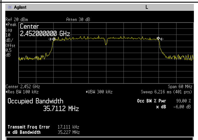
802.11n40 6dB Bandwidth - High CH 2452
