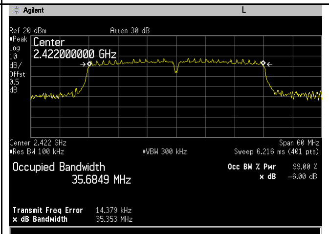
802.11n40 6dB Bandwidth - Low CH 2422
