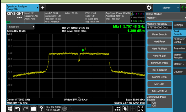
Channel 159 (5795MHz)
