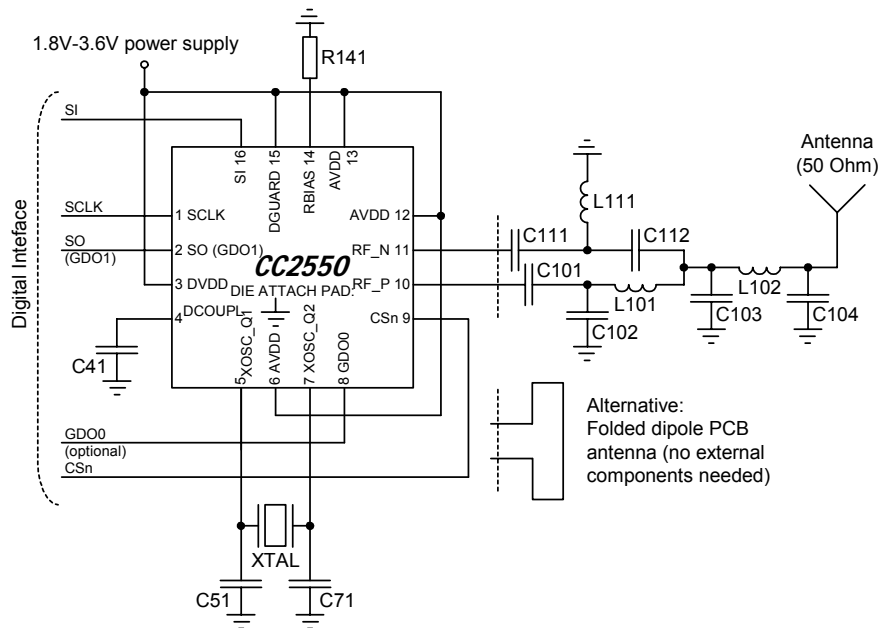
Figure 3: Typical application and evaluation circuit (power supply decoupling not shown)
