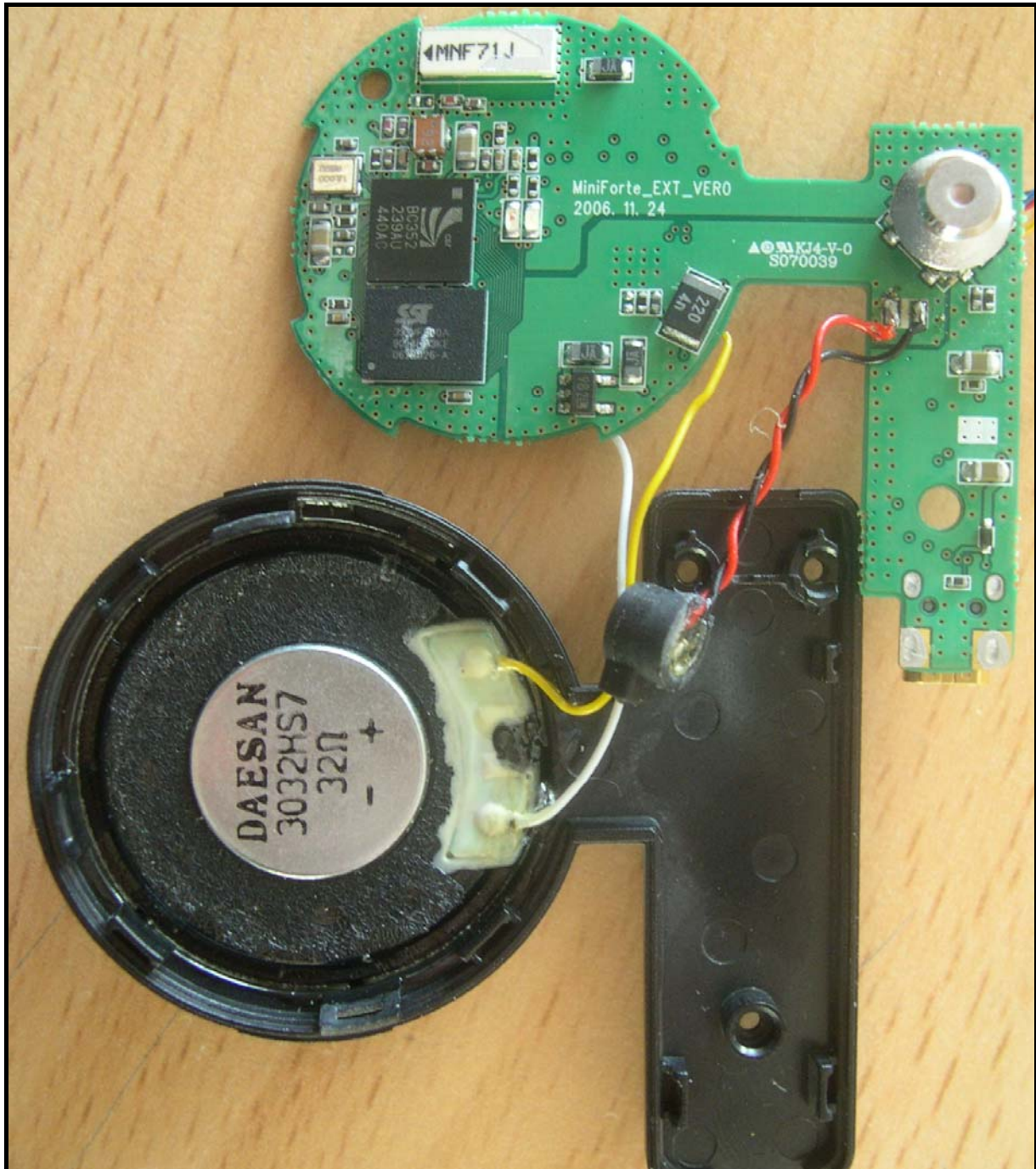
<Photograph 1: Internal Front View_Main Board>
