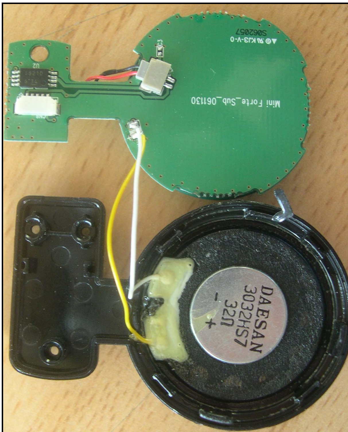
<Photograph 3: Internal Rear View_Sub Board>
