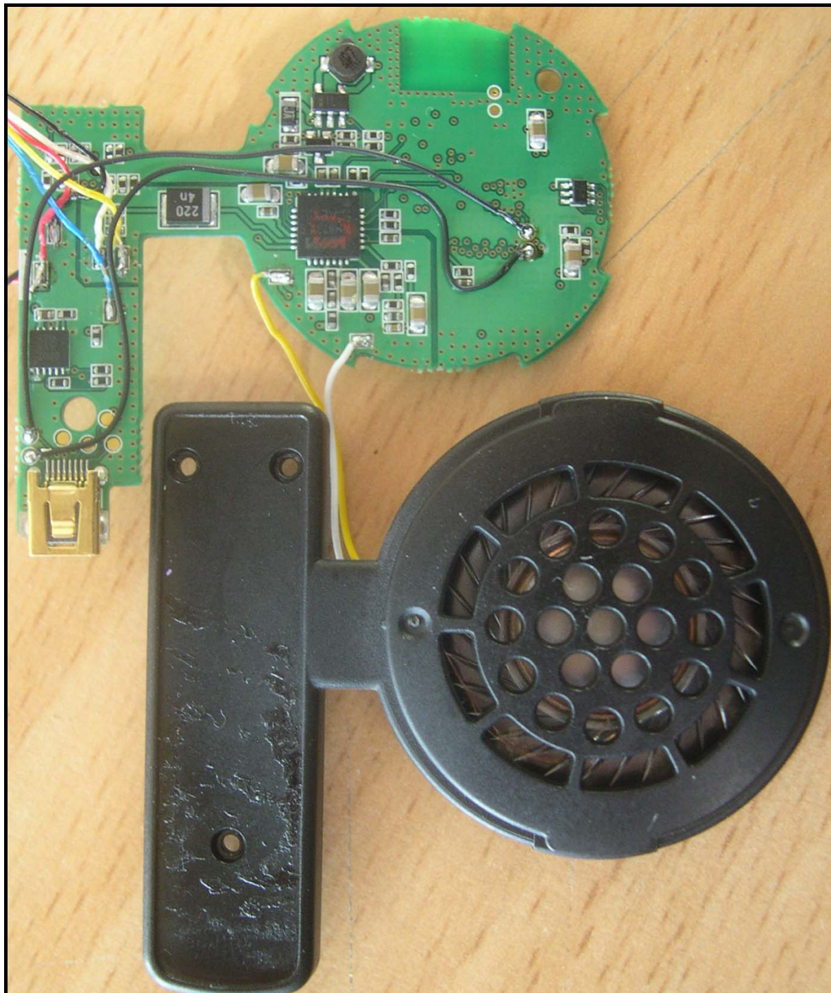
<Photograph 2: Internal Rear View_Main Board>
