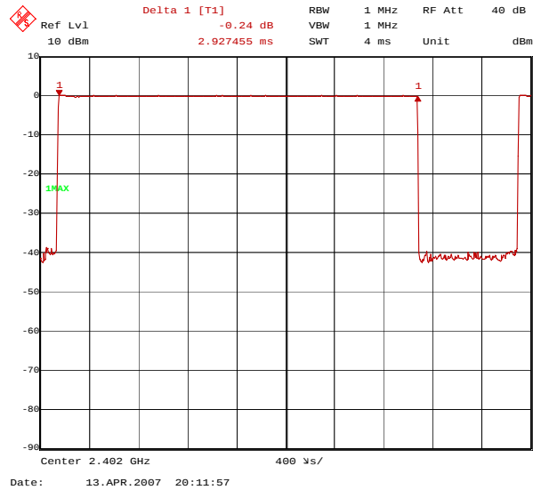
Figure 5. Plot of the Time of Occupancy (Conducted)
