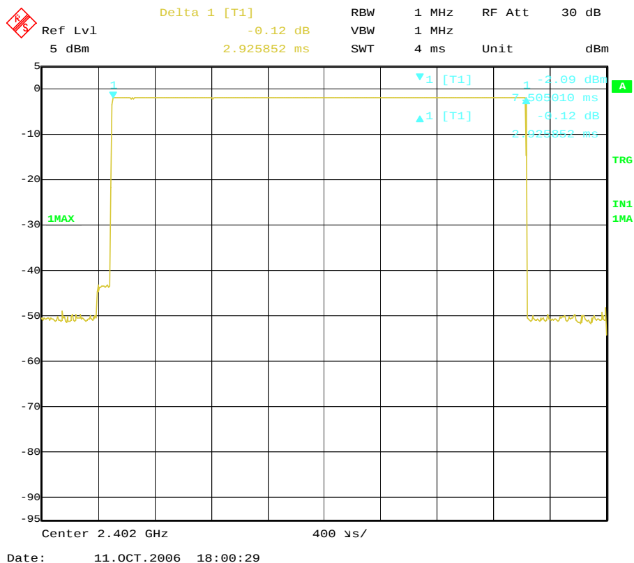
Figure 5. Plot of the Time of Occupancy (Conducted)
