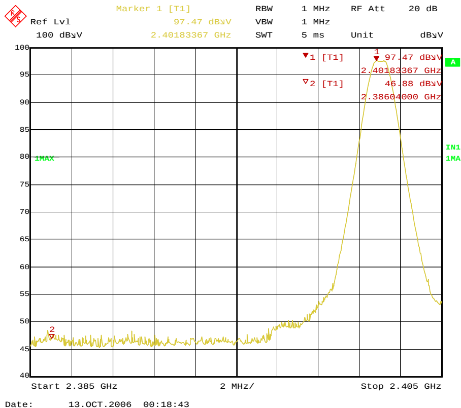
Figure 7. Plot of the Band Edge (Radiated)
