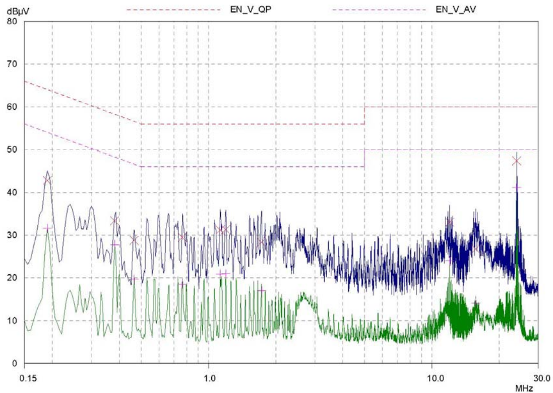
Figure 10. Plot of the Conducted Emissions
