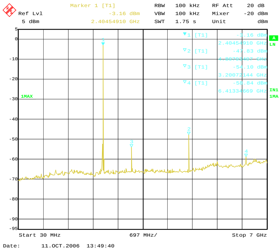
Figure 8. Plot of the RF antenna port emissions (Conducted)
