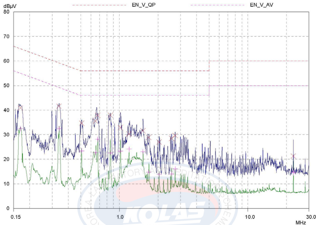
Figure 10. Plot of the AC Power Line Conducted Emissions ( \pi/4 DQPSK )
