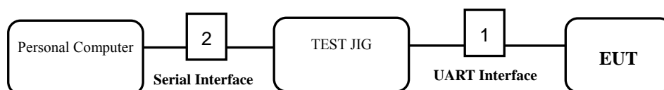
[ System Block Diagram of Test Configuration ]
