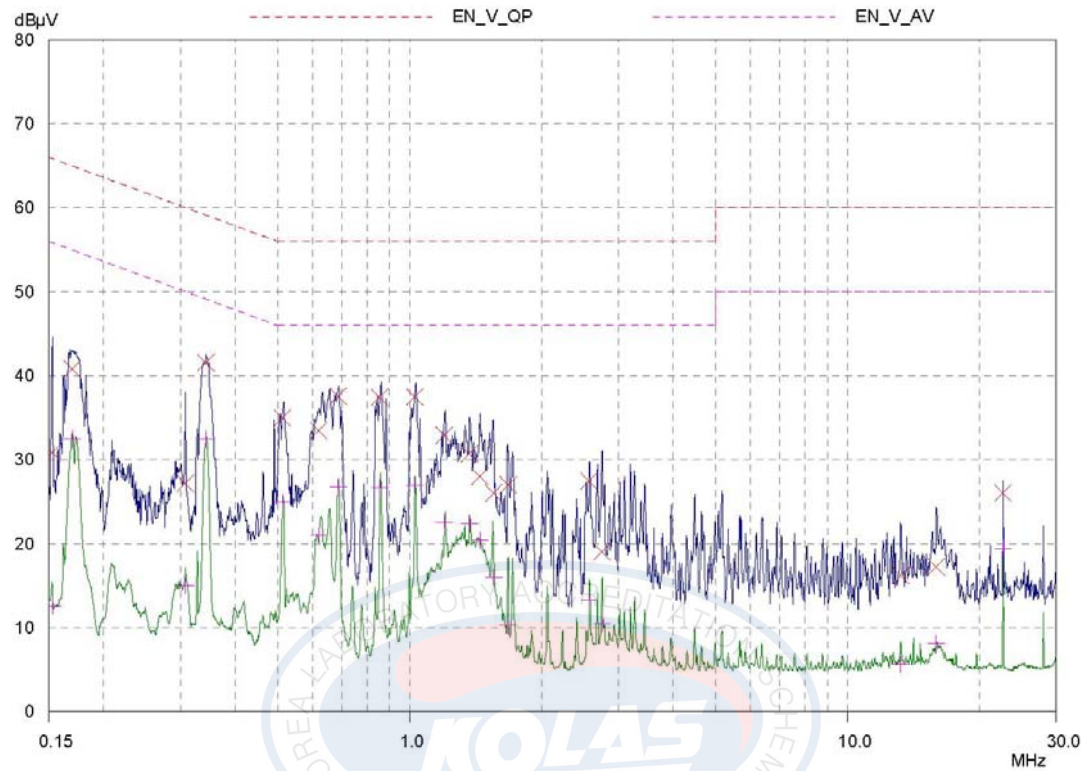
Figure 10. Plot of the AC Power Line Conducted Emissions ( GFSK )
