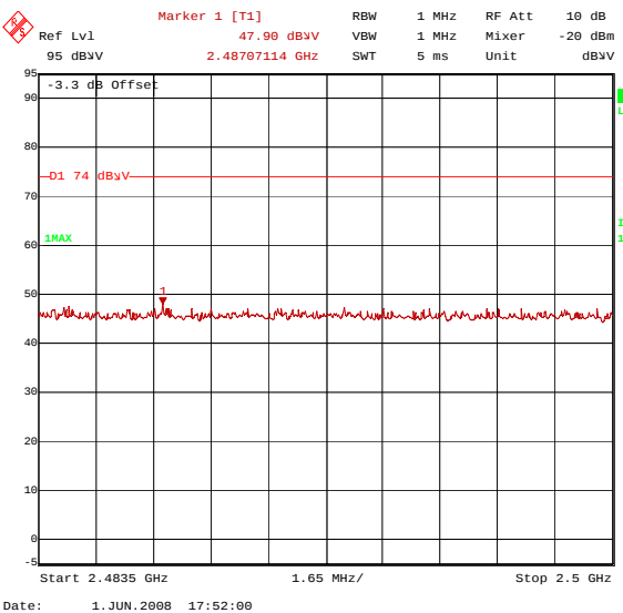
Figure 7. Plot of the Band Edge (Radiated) GFSK Modulation π / 4 DQPSK Modulation Highest Channel (operating at 2480 MHz): PEAK
