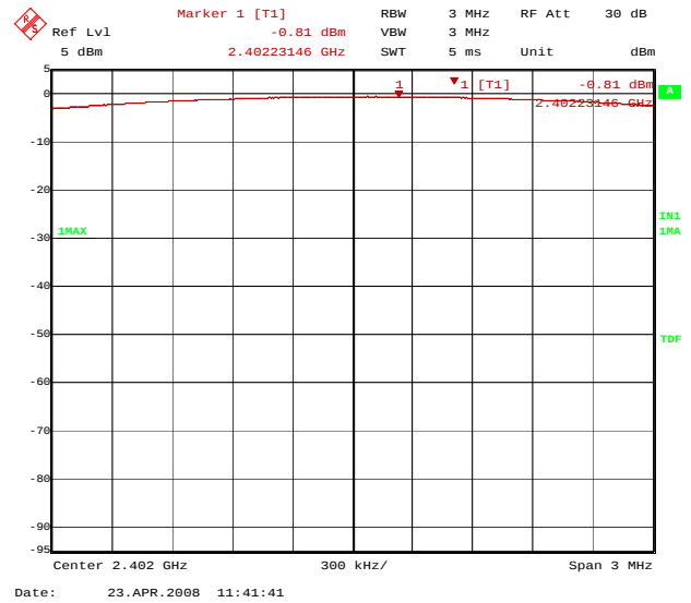
Figure 1. Plot of the Maximum Peak Output Power (Conducted) GFSK Modulation Lowest Channel(2402 MHz)
