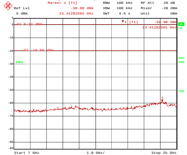
Figure 8: Spurious RF conducted emissions__ GFSK Modulation
