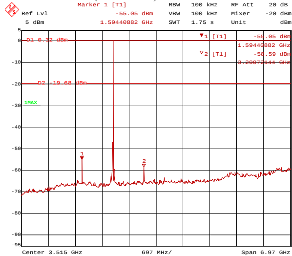
Figure 8: Spurious RF conducted emissions__ GFSK Modulation
